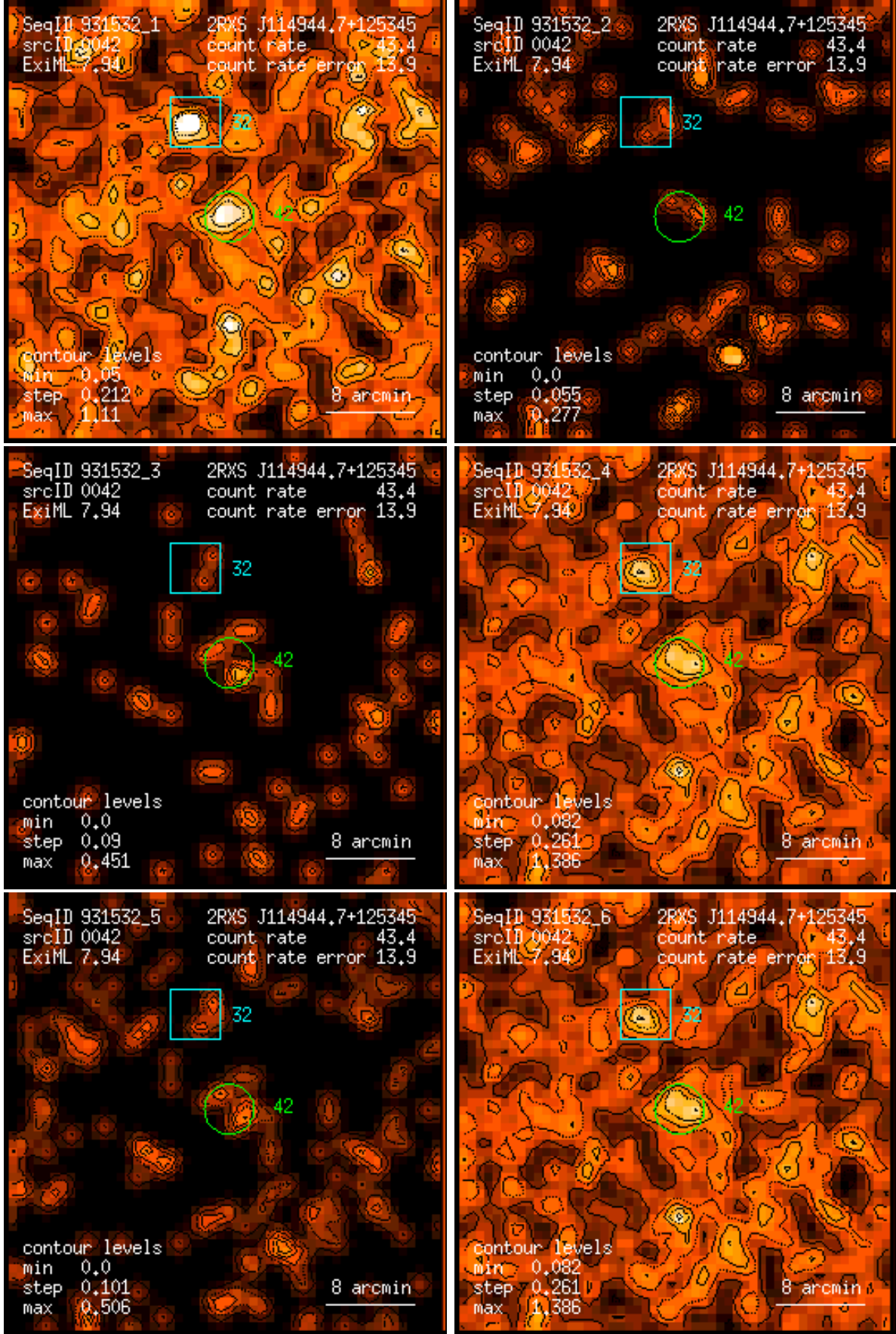
Figure 42: RASS 931532: detection 0042: band rate images, Gaussian filter: (1) PSPC channels 11 – 41, (2) 52 – 90, (3) 91 – 201, (4) 11 – 235, (5) 52 – 201, (6) 11 – 201. Broad band rates in counts/ks. Band rate contour levels in counts/ks/arcmin 2 .
