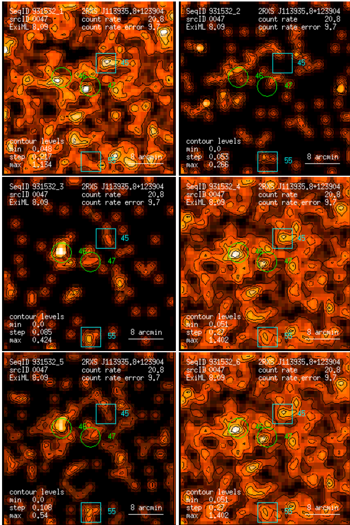
Figure 47: RASS 931532: detection 0047: band rate images, Gaussian filter: (1) PSPC channels 11 – 41, (2) 52 – 90, (3) 91 – 201, (4) 11 – 235, (5) 52 – 201, (6) 11 – 201. Broad band rates in counts/ks. Band rate contour levels in counts/ks/arcmin 2 .
