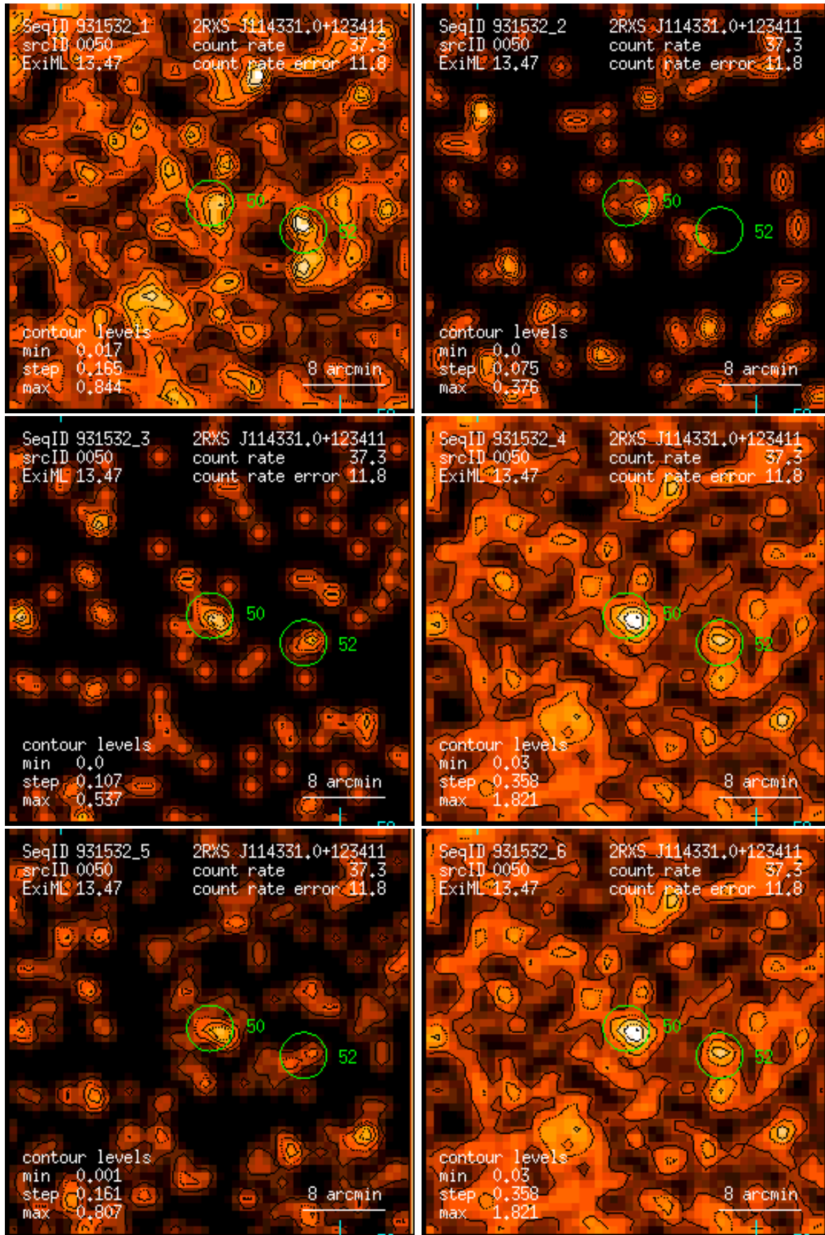
Figure 50: RASS 931532: detection 0050: band rate images, Gaussian filter: (1) PSPC channels 11 – 41, (2) 52 – 90, (3) 91 – 201, (4) 11 – 235, (5) 52 – 201, (6) 11 – 201. Broad band rates in counts/ks. Band rate contour levels in counts/ks/arcmin 2 .
