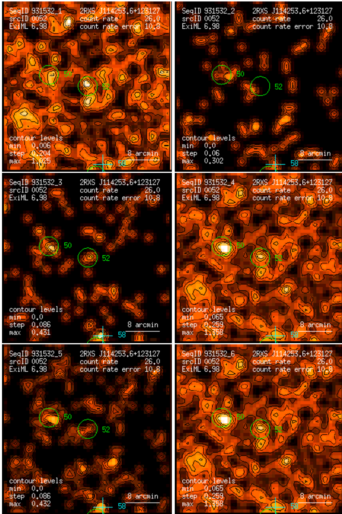
Figure 52: RASS 931532: detection 0052: band rate images, Gaussian filter: (1) PSPC channels 11 – 41, (2) 52 – 90, (3) 91 – 201, (4) 11 – 235, (5) 52 – 201, (6) 11 – 201. Broad band rates in counts/ks. Band rate contour levels in counts/ks/arcmin 2 .
