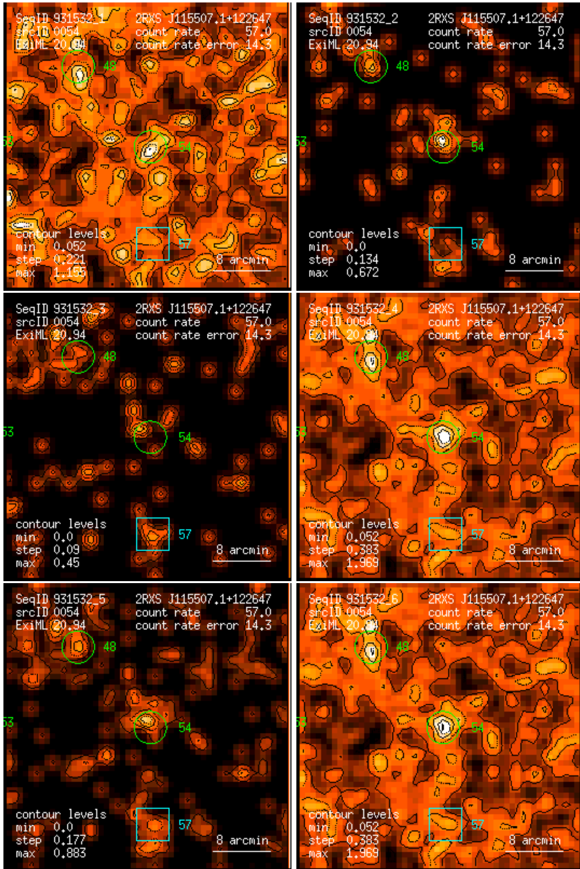
Figure 54: RASS 931532: detection 0054: band rate images, Gaussian filter: (1) PSPC channels 11 – 41, (2) 52 – 90, (3) 91 – 201, (4) 11 – 235, (5) 52 – 201, (6) 11 – 201. Broad band rates in counts/ks. Band rate contour levels in counts/ks/arcmin 2 .
