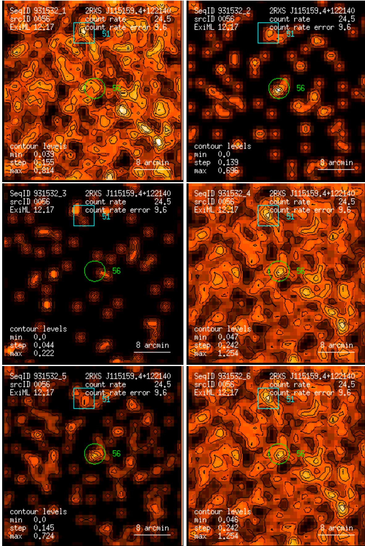
Figure 56: RASS 931532: detection 0056: band rate images, Gaussian filter: (1) PSPC channels 11 – 41, (2) 52 – 90, (3) 91 – 201, (4) 11 – 235, (5) 52 – 201, (6) 11 – 201. Broad band rates in counts/ks. Band rate contour levels in counts/ks/arcmin 2 .
