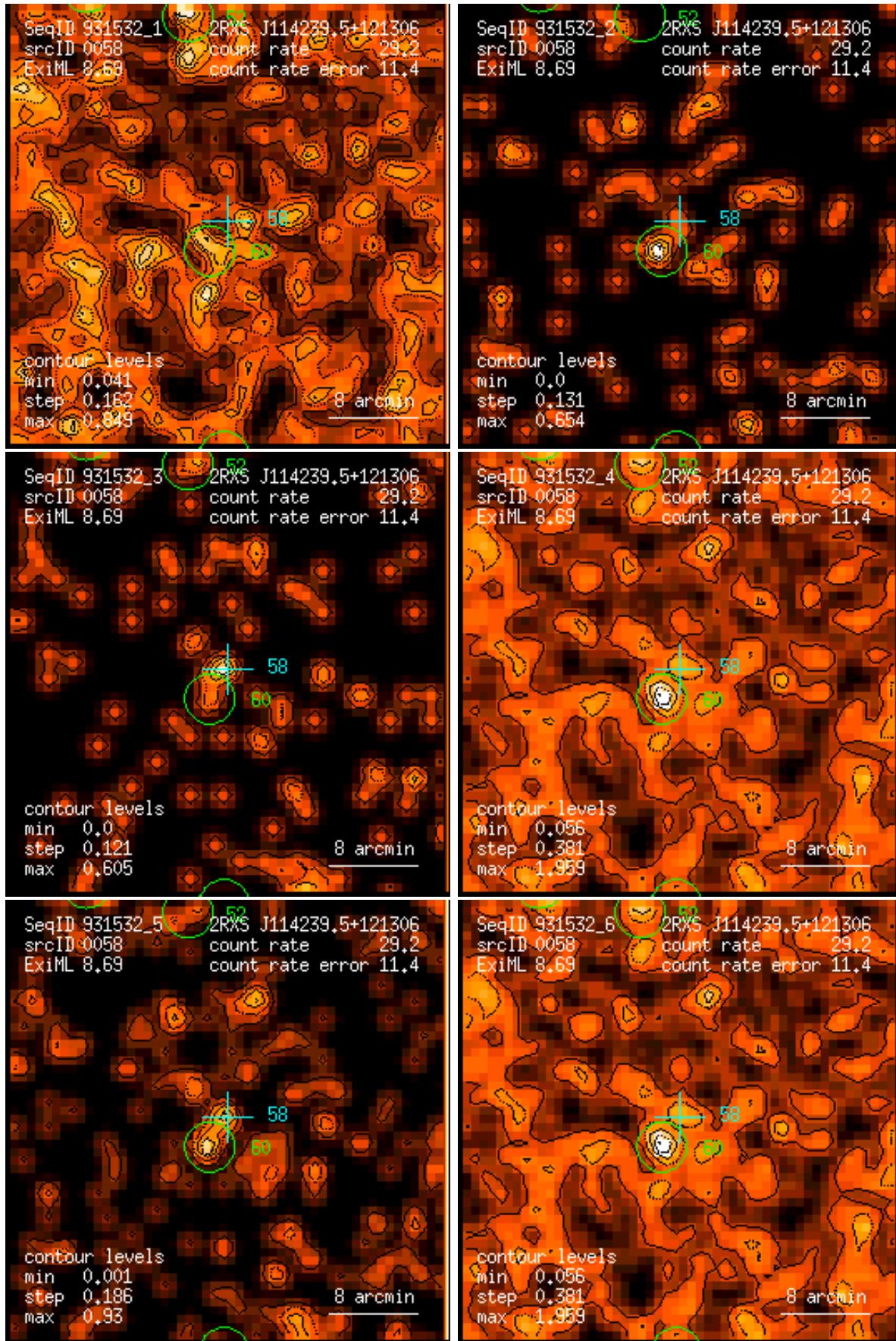
Figure 58: RASS 931532: detection 0058: band rate images, Gaussian filter: (1) PSPC channels 11 – 41, (2) 52 – 90, (3) 91 – 201, (4) 11 – 235, (5) 52 – 201, (6) 11 – 201. Broad band rates in counts/ks. Band rate contour levels in counts/ks/arcmin 2 .
