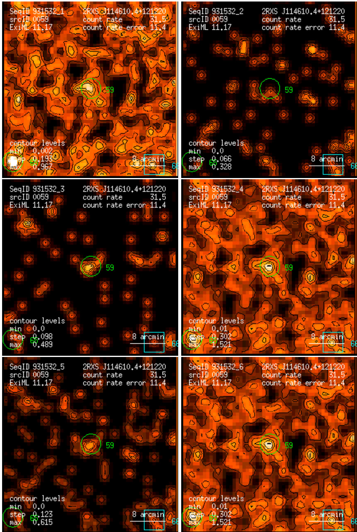
Figure 59: RASS 931532: detection 0059: band rate images, Gaussian filter: (1) PSPC channels 11 – 41, (2) 52 – 90, (3) 91 – 201, (4) 11 – 235, (5) 52 – 201, (6) 11 – 201. Broad band rates in counts/ks. Band rate contour levels in counts/ks/arcmin 2 .
