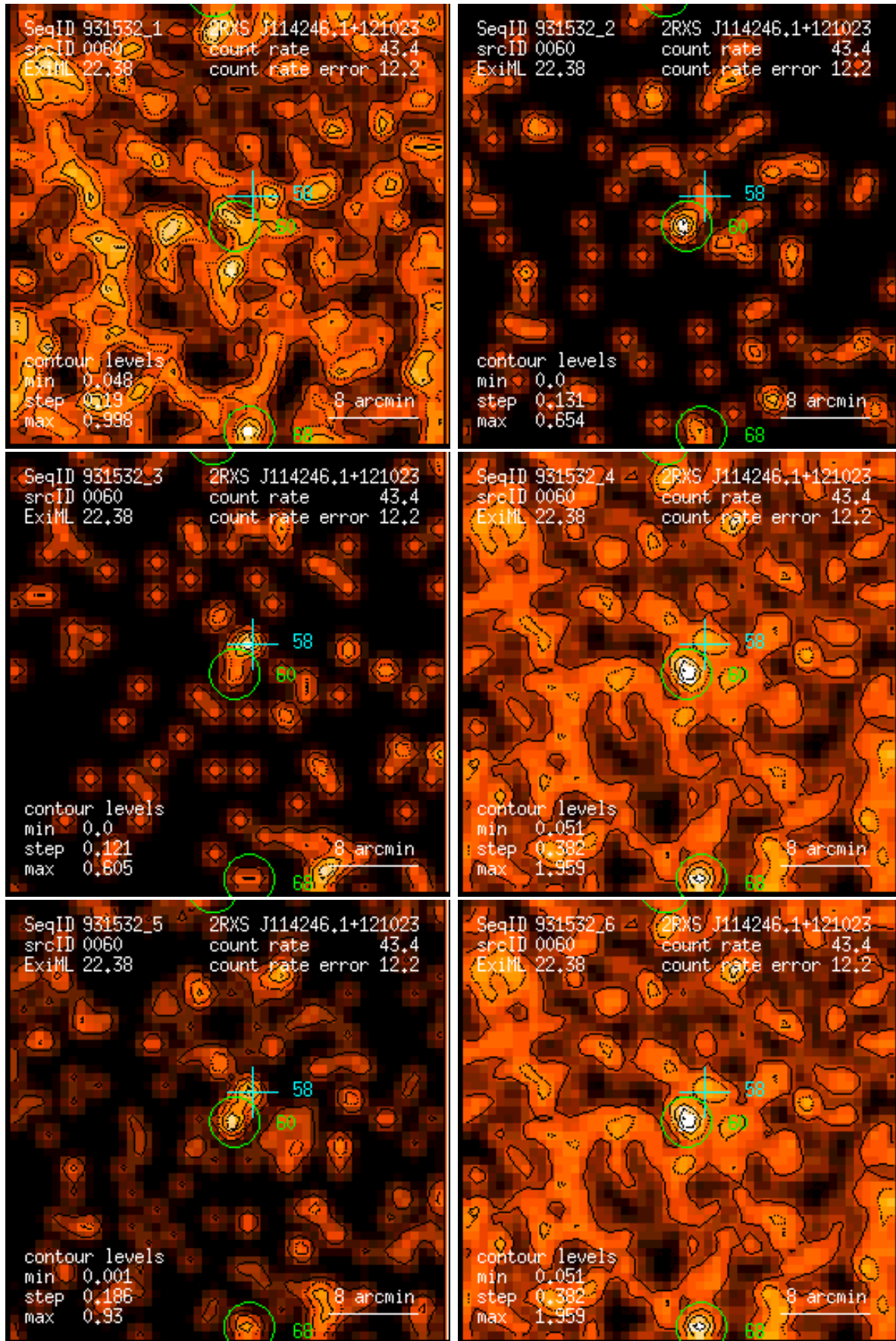
Figure 60: RASS 931532: detection 0060: band rate images, Gaussian filter: (1) PSPC channels 11 – 41, (2) 52 – 90, (3) 91 – 201, (4) 11 – 235, (5) 52 – 201, (6) 11 – 201. Broad band rates in counts/ks. Band rate contour levels in counts/ks/arcmin 2 .
