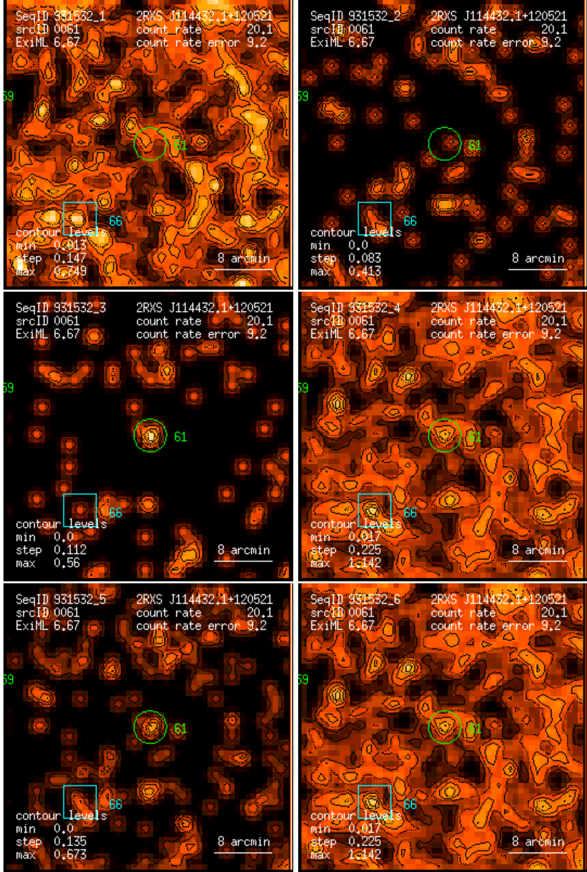
Figure 61: RASS 931532: detection 0061: band rate images, Gaussian filter: (1) PSPC channels 11 – 41, (2) 52 – 90, (3) 91 – 201, (4) 11 – 235, (5) 52 – 201, (6) 11 – 201. Broad band rates in counts/ks. Band rate contour levels in counts/ks/arcmin 2 .
