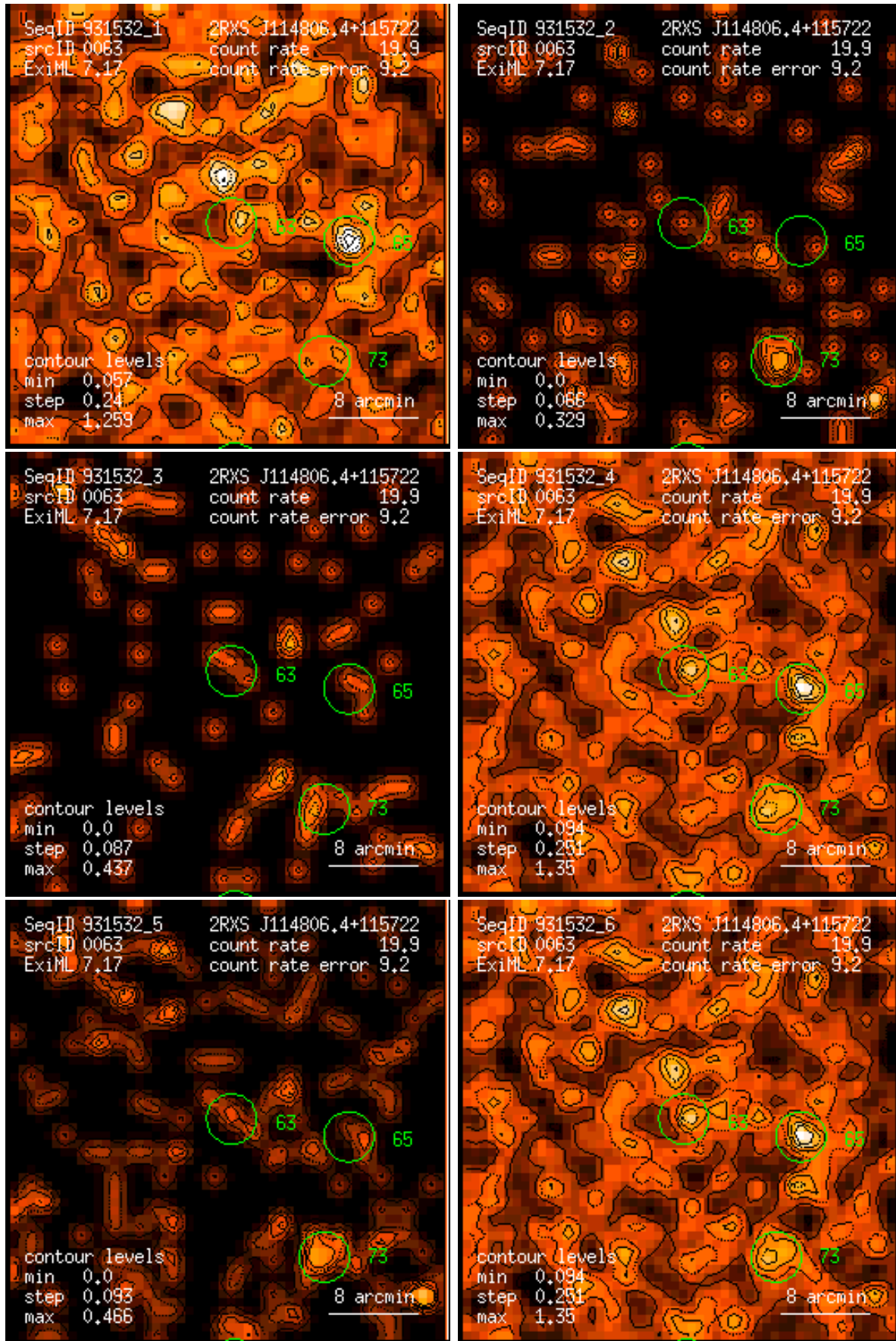
Figure 63: RASS 931532: detection 0063: band rate images, Gaussian filter: (1) PSPC channels 11 – 41, (2) 52 – 90, (3) 91 – 201, (4) 11 – 235, (5) 52 – 201, (6) 11 – 201. Broad band rates in counts/ks. Band rate contour levels in counts/ks/arcmin 2 .
