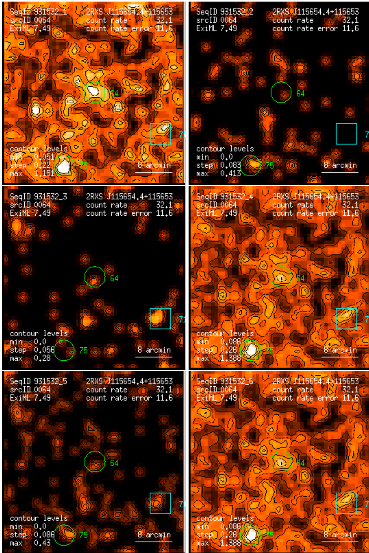
Figure 64: RASS 931532: detection 0064: band rate images, Gaussian filter: (1) PSPC channels 11 – 41, (2) 52 – 90, (3) 91 – 201, (4) 11 – 235, (5) 52 – 201, (6) 11 – 201. Broad band rates in counts/ks. Band rate contour levels in counts/ks/arcmin 2 .
