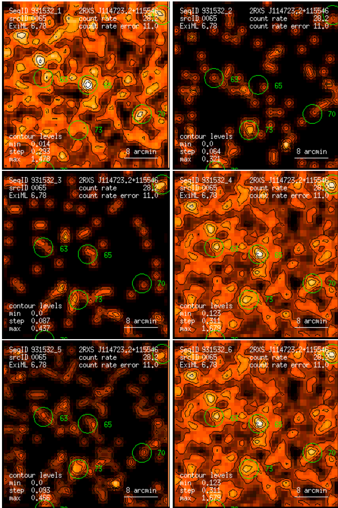
Figure 65: RASS 931532: detection 0065: band rate images, Gaussian filter: (1) PSPC channels 11 – 41, (2) 52 – 90, (3) 91 – 201, (4) 11 – 235, (5) 52 – 201, (6) 11 – 201. Broad band rates in counts/ks. Band rate contour levels in counts/ks/arcmin 2 .
