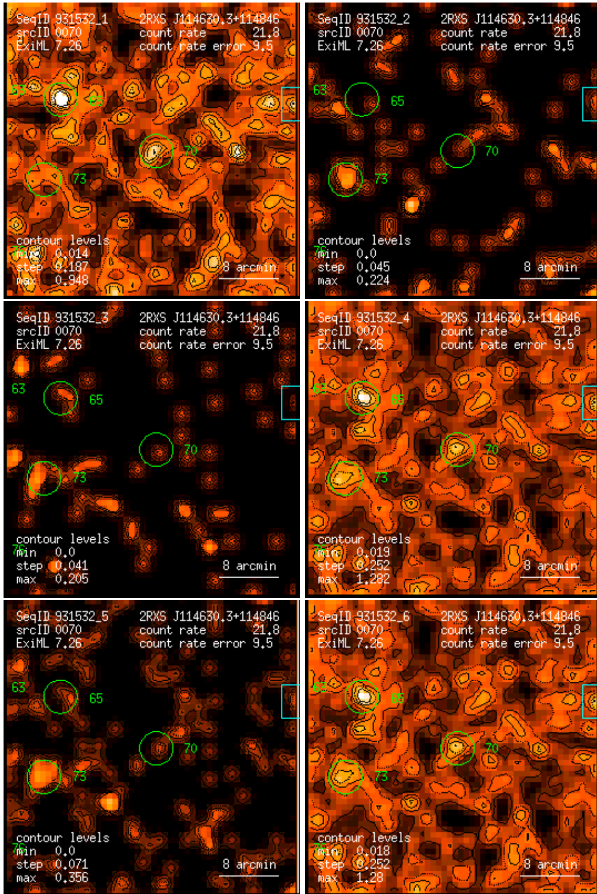
Figure 70: RASS 931532: detection 0070: band rate images, Gaussian filter: (1) PSPC channels 11 – 41, (2) 52 – 90, (3) 91 – 201, (4) 11 – 235, (5) 52 – 201, (6) 11 – 201. Broad band rates in counts/ks. Band rate contour levels in counts/ks/arcmin 2 .
