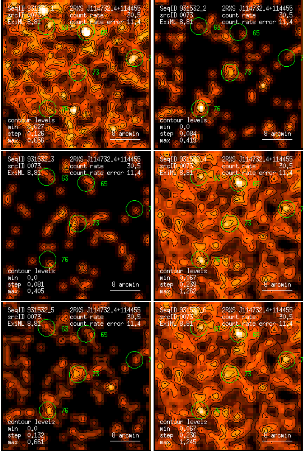
Figure 73: RASS 931532: detection 0073: band rate images, Gaussian filter: (1) PSPC channels 11 – 41, (2) 52 – 90, (3) 91 – 201, (4) 11 – 235, (5) 52 – 201, (6) 11 – 201. Broad band rates in counts/ks. Band rate contour levels in counts/ks/arcmin 2 .
