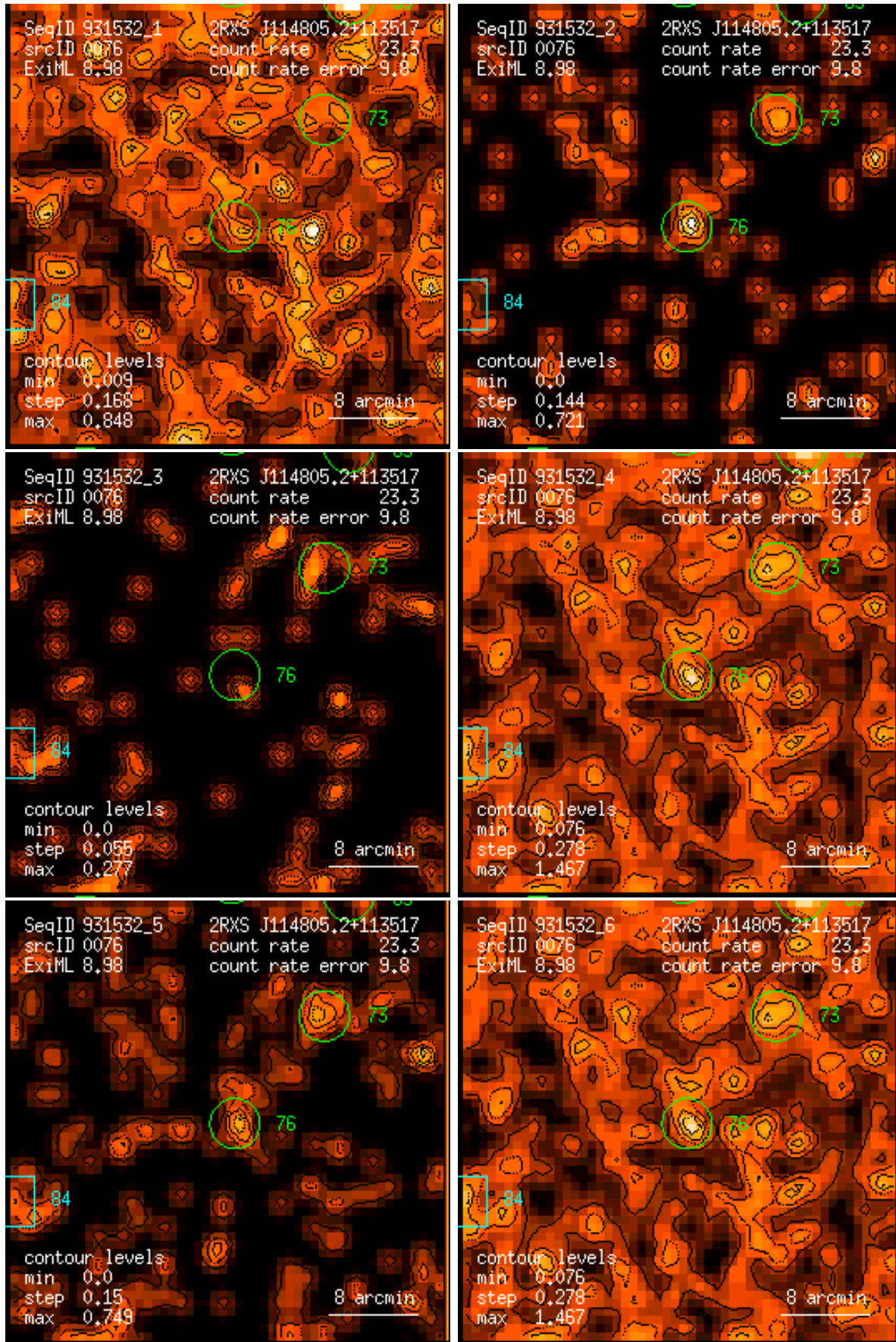
Figure 76: RASS 931532: detection 0076: band rate images, Gaussian filter: (1) PSPC channels 11 – 41, (2) 52 – 90, (3) 91 – 201, (4) 11 – 235, (5) 52 – 201, (6) 11 – 201. Broad band rates in counts/ks. Band rate contour levels in counts/ks/arcmin 2 .
