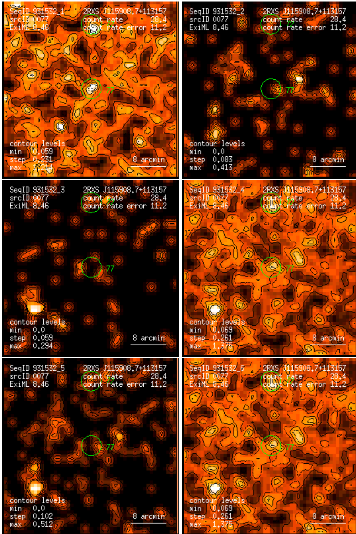
Figure 77: RASS 931532: detection 0077: band rate images, Gaussian filter: (1) PSPC channels 11 – 41, (2) 52 – 90, (3) 91 – 201, (4) 11 – 235, (5) 52 – 201, (6) 11 – 201. Broad band rates in counts/ks. Band rate contour levels in counts/ks/arcmin 2 .
