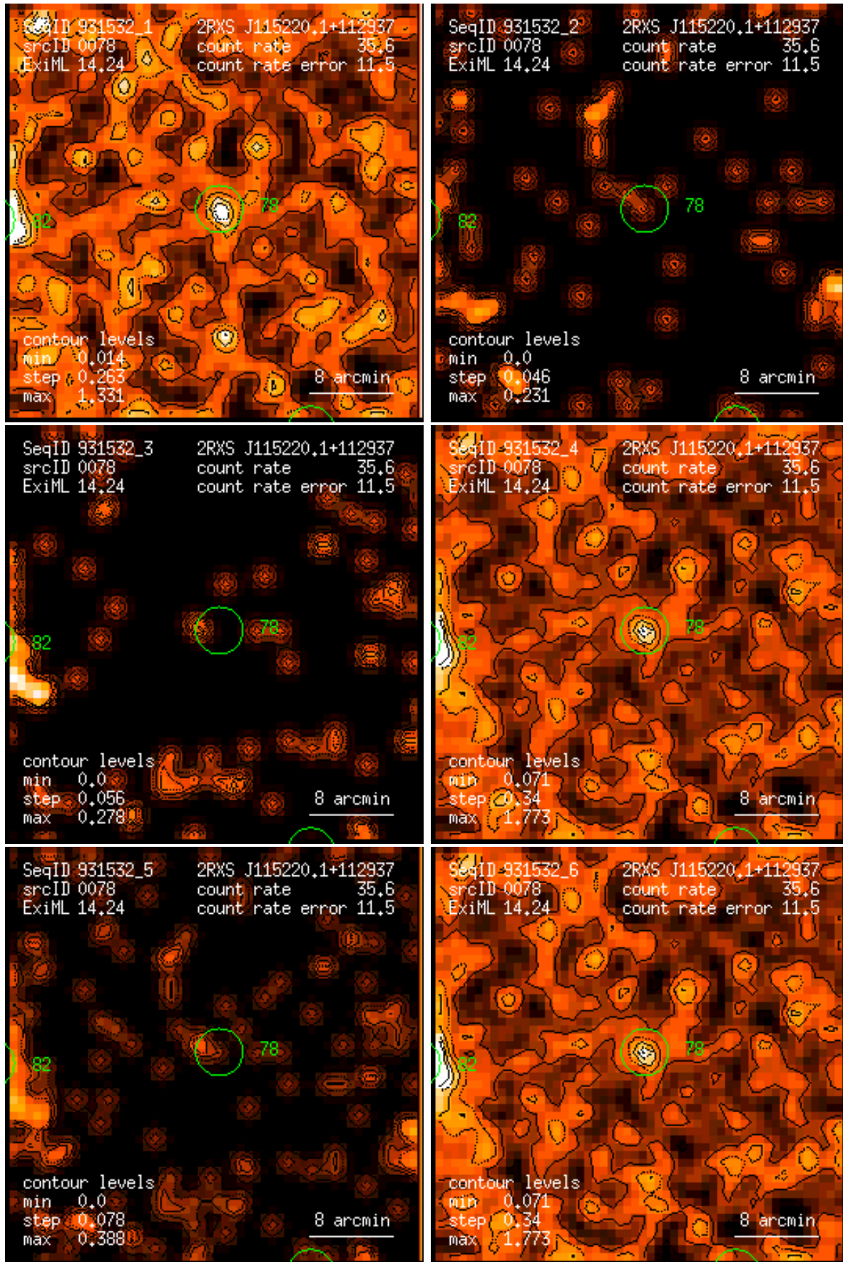
Figure 78: RASS 931532: detection 0078: band rate images, Gaussian filter: (1) PSPC channels 11 – 41, (2) 52 – 90, (3) 91 – 201, (4) 11 – 235, (5) 52 – 201, (6) 11 – 201. Broad band rates in counts/ks. Band rate contour levels in counts/ks/arcmin 2 .
