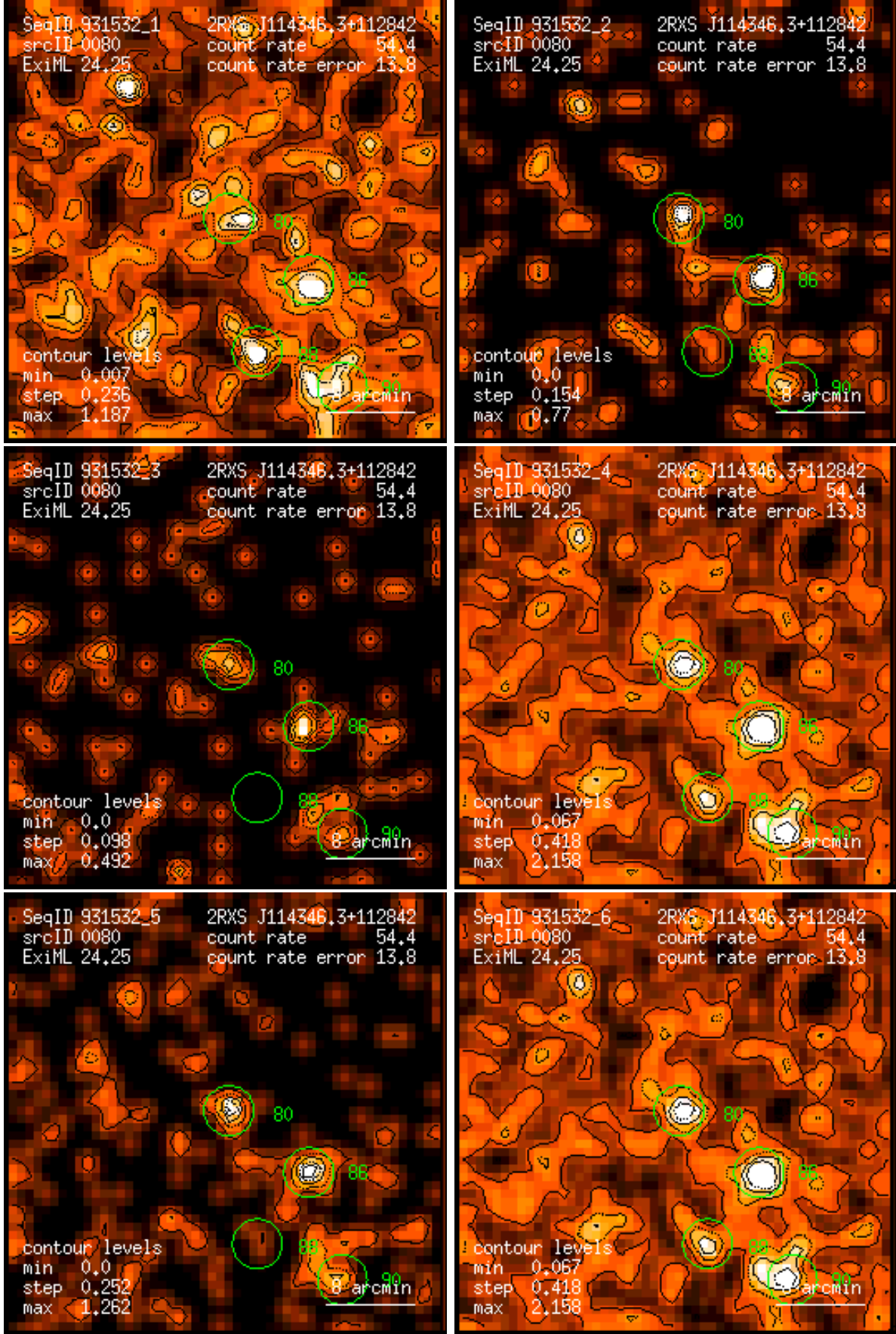
Figure 80: RASS 931532: detection 0080: band rate images, Gaussian filter: (1) PSPC channels 11 – 41, (2) 52 – 90, (3) 91 – 201, (4) 11 – 235, (5) 52 – 201, (6) 11 – 201. Broad band rates in counts/ks. Band rate contour levels in counts/ks/arcmin 2 .
