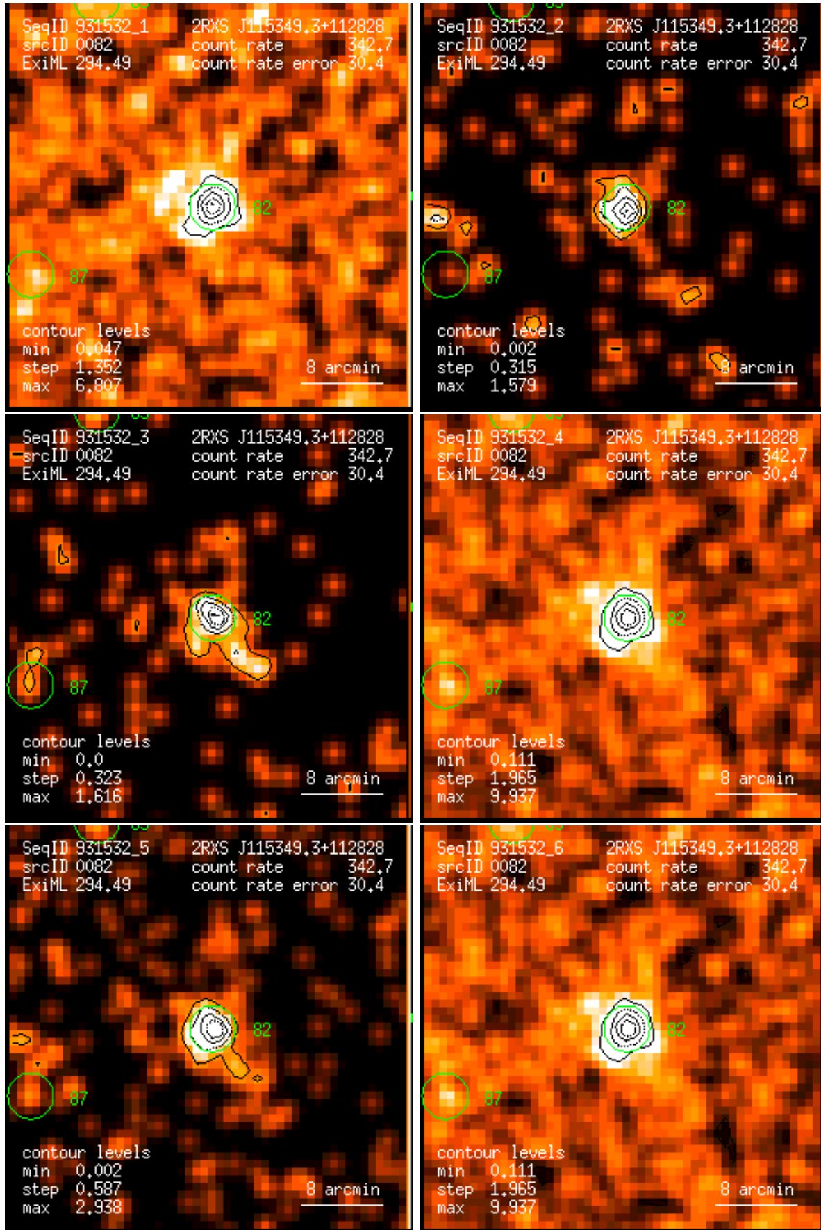
Figure 82: RASS 931532: detection 0082: band rate images, Gaussian filter: (1) PSPC channels 11 – 41, (2) 52 – 90, (3) 91 – 201, (4) 11 – 235, (5) 52 – 201, (6) 11 – 201. Broad band rates in counts/ks. Band rate contour levels in counts/ks/arcmin 2 .
