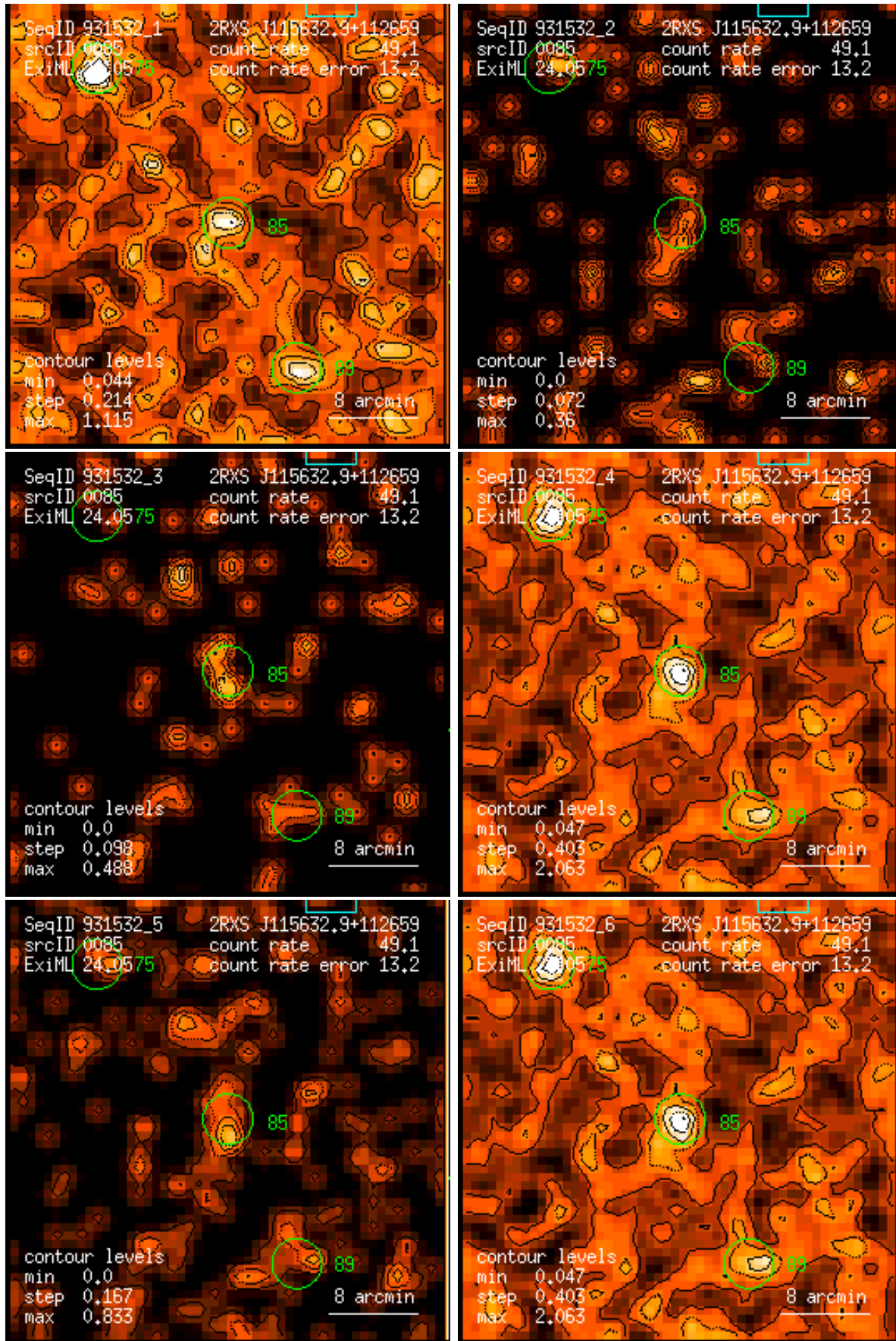
Figure 85: RASS 931532: detection 0085: band rate images, Gaussian filter: (1) PSPC channels 11 – 41, (2) 52 – 90, (3) 91 – 201, (4) 11 – 235, (5) 52 – 201, (6) 11 – 201. Broad band rates in counts/ks. Band rate contour levels in counts/ks/arcmin 2 .
