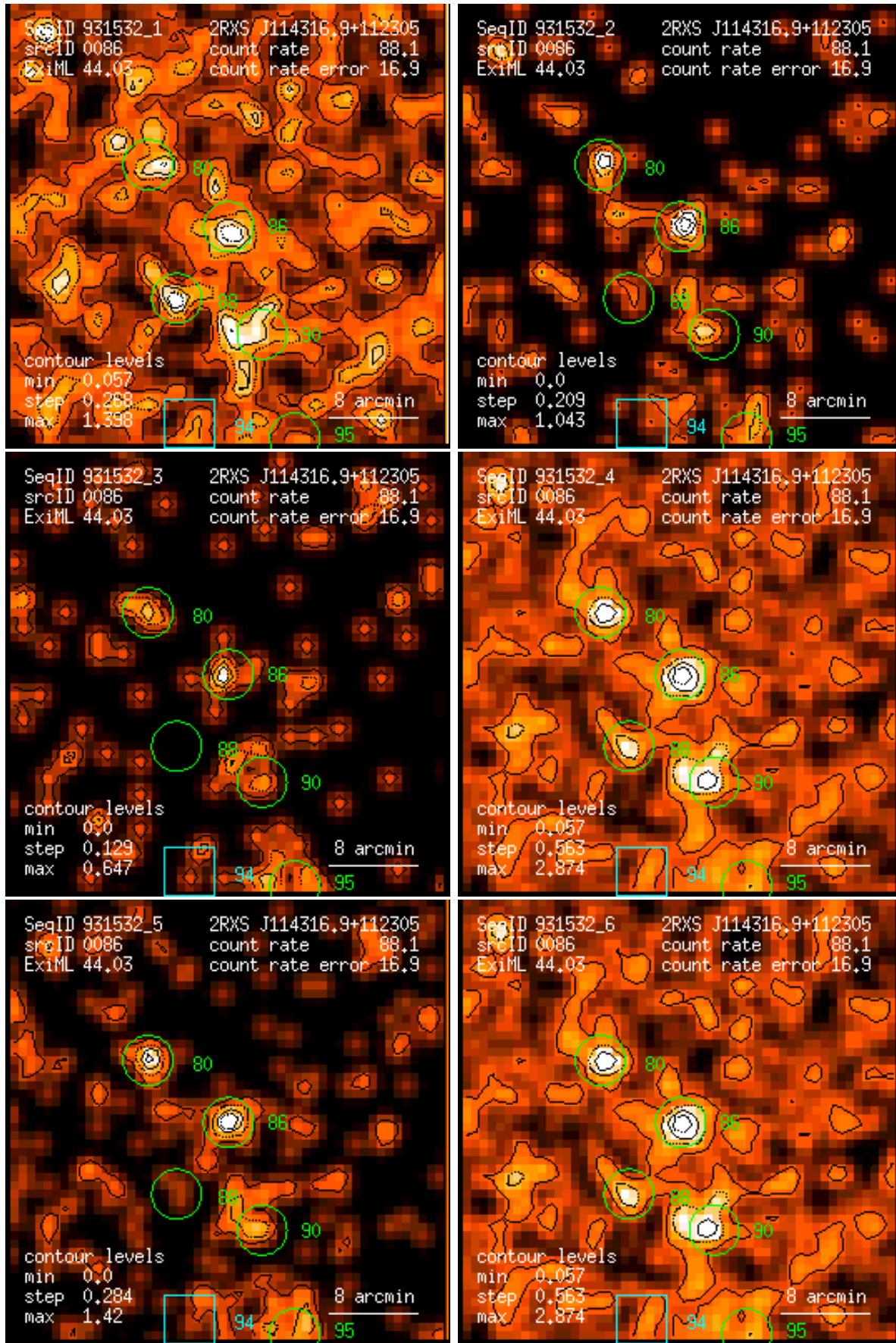
Figure 86: RASS 931532: detection 0086: band rate images, Gaussian filter: (1) PSPC channels 11 – 41, (2) 52 – 90, (3) 91 – 201, (4) 11 – 235, (5) 52 – 201, (6) 11 – 201. Broad band rates in counts/ks. Band rate contour levels in counts/ks/arcmin 2 .
