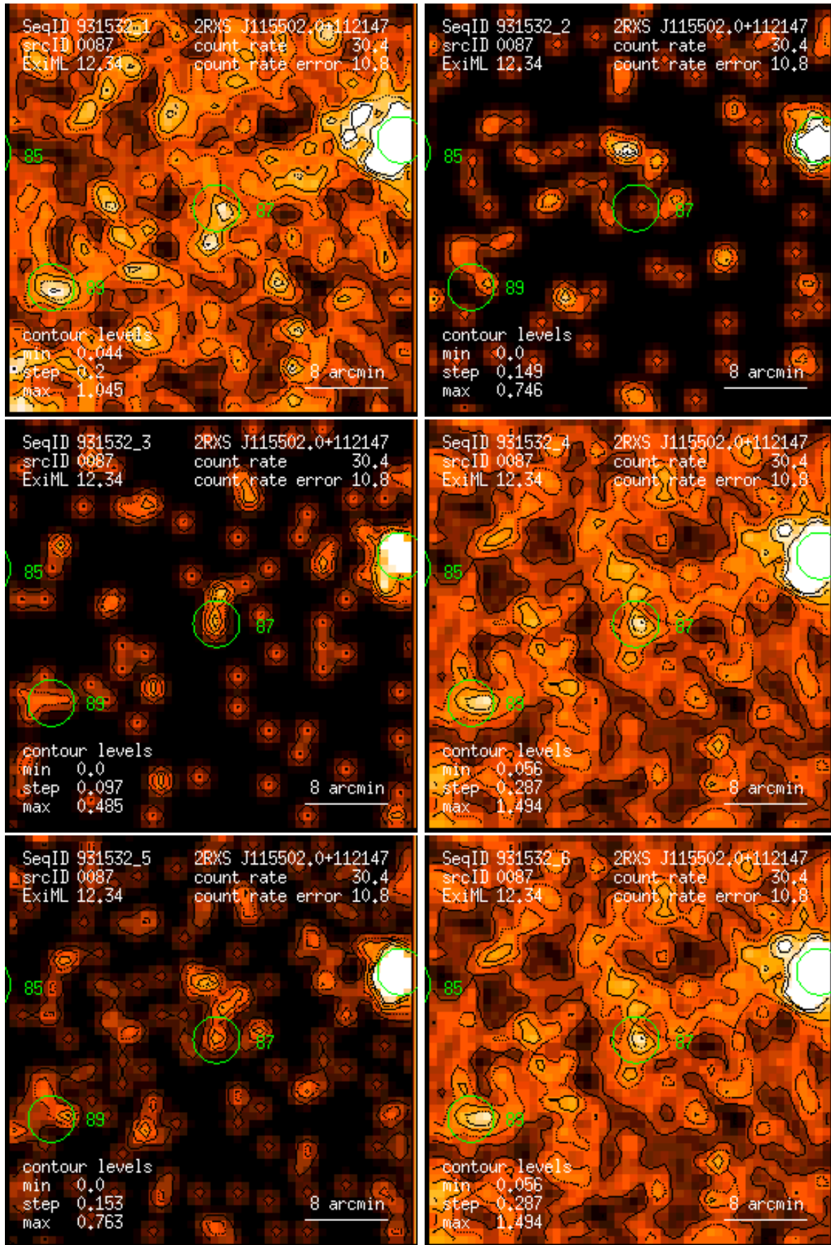
Figure 87: RASS 931532: detection 0087: band rate images, Gaussian filter: (1) PSPC channels 11 – 41, (2) 52 – 90, (3) 91 – 201, (4) 11 – 235, (5) 52 – 201, (6) 11 – 201. Broad band rates in counts/ks. Band rate contour levels in counts/ks/arcmin 2 .
