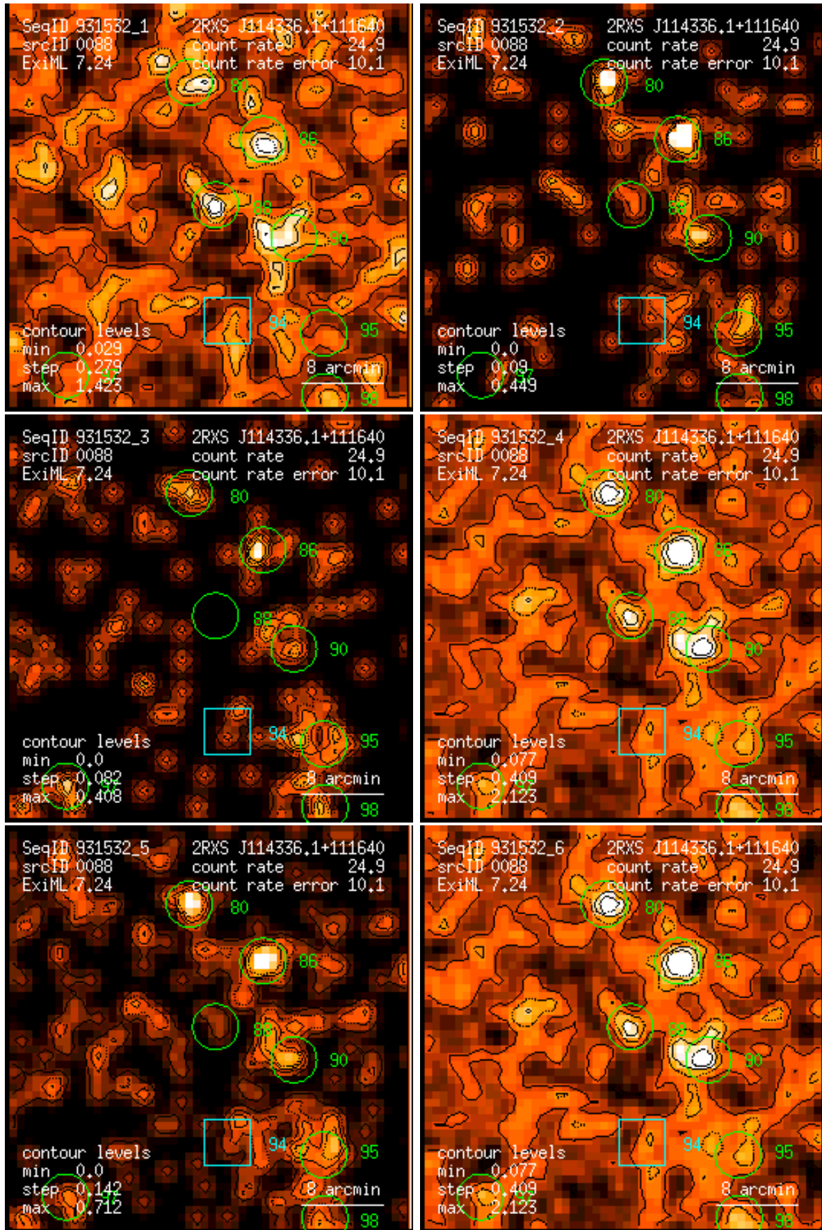
Figure 88: RASS 931532: detection 0088: band rate images, Gaussian filter: (1) PSPC channels 11 – 41, (2) 52 – 90, (3) 91 – 201, (4) 11 – 235, (5) 52 – 201, (6) 11 – 201. Broad band rates in counts/ks. Band rate contour levels in counts/ks/arcmin 2 .
