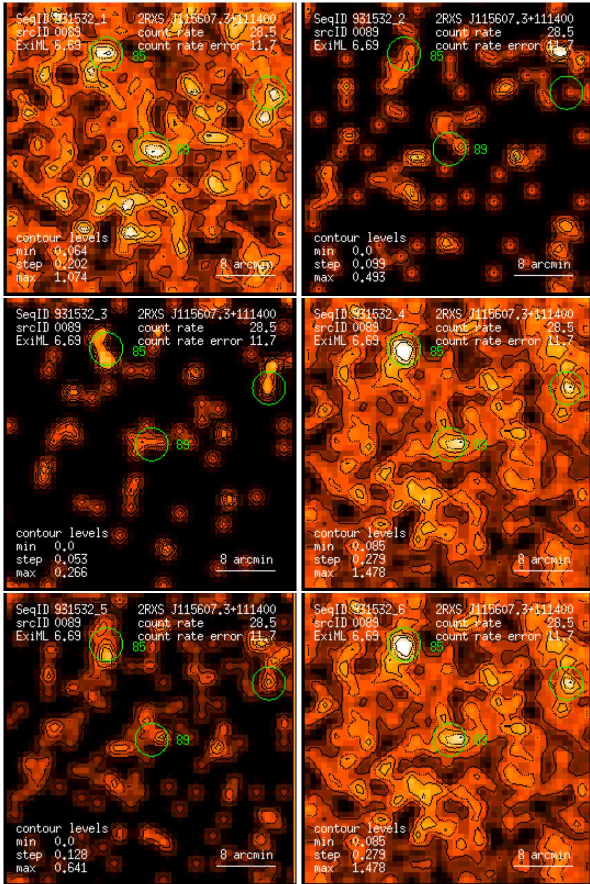
Figure 89: RASS 931532: detection 0089: band rate images, Gaussian filter: (1) PSPC channels 11 – 41, (2) 52 – 90, (3) 91 – 201, (4) 11 – 235, (5) 52 – 201, (6) 11 – 201. Broad band rates in counts/ks. Band rate contour levels in counts/ks/arcmin 2 .
