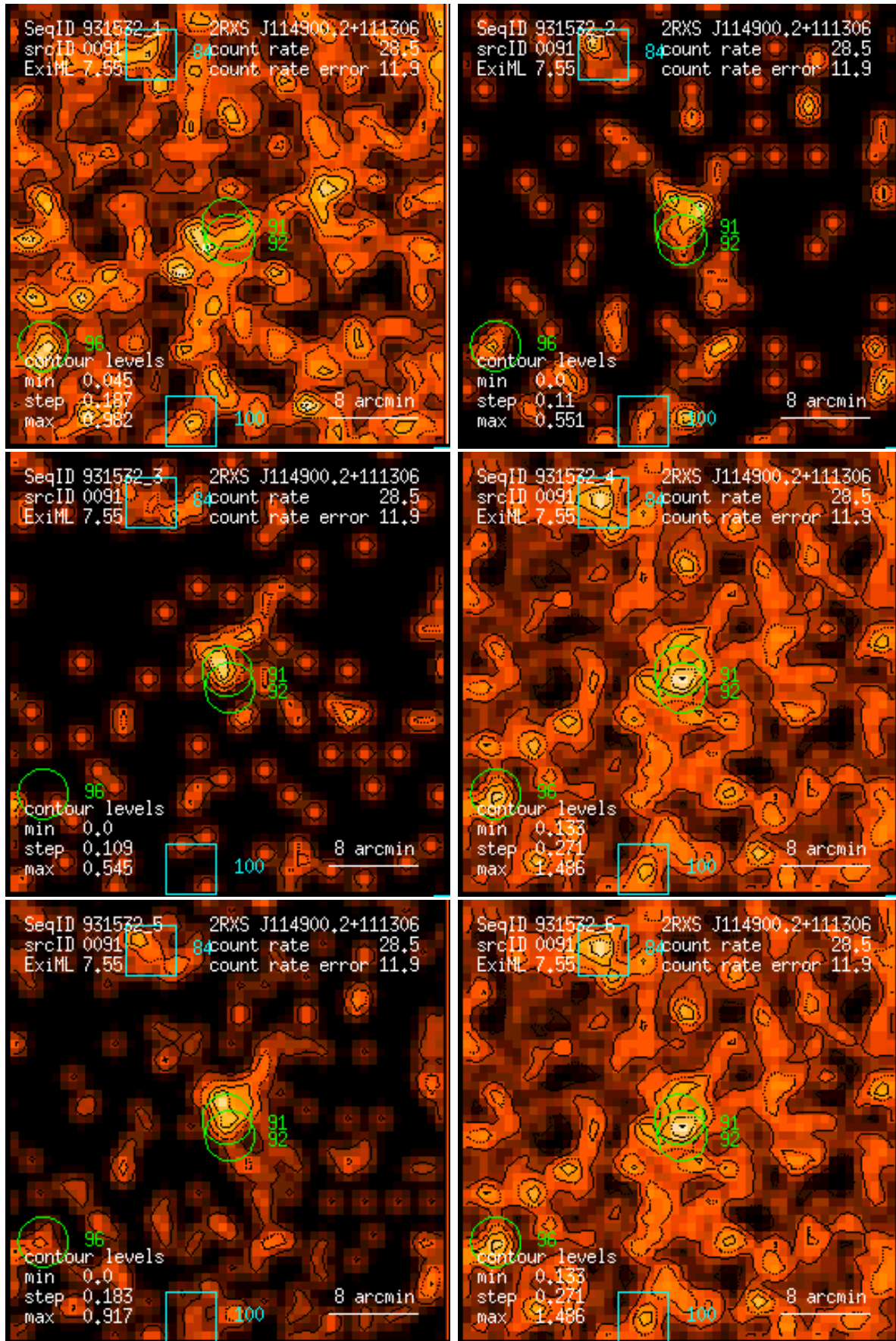
Figure 91: RASS 931532: detection 0091: band rate images, Gaussian filter: (1) PSPC channels 11 – 41, (2) 52 – 90, (3) 91 – 201, (4) 11 – 235, (5) 52 – 201, (6) 11 – 201. Broad band rates in counts/ks. Band rate contour levels in counts/ks/arcmin 2 .
