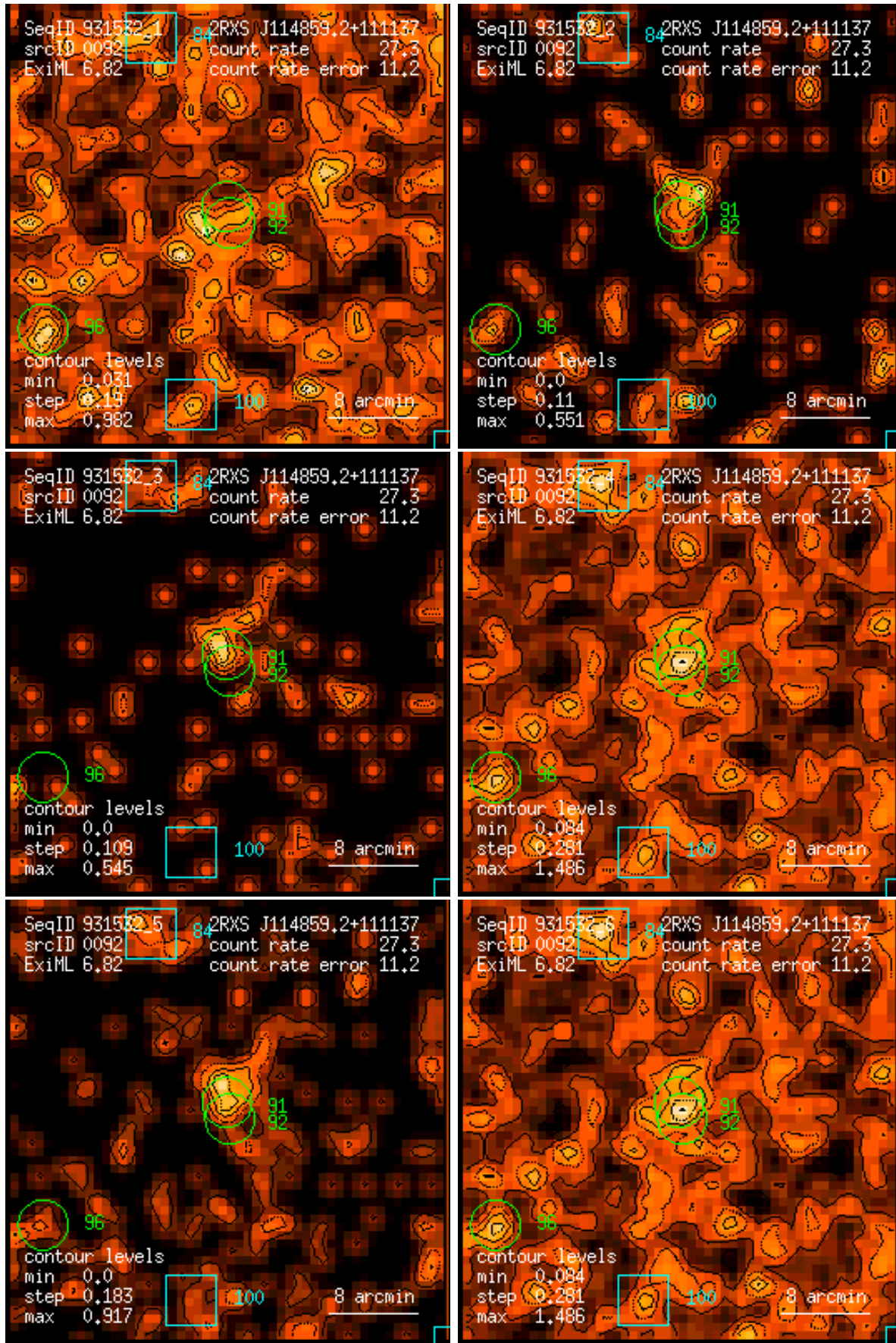
Figure 92: RASS 931532: detection 0092: band rate images, Gaussian filter: (1) PSPC channels 11 – 41, (2) 52 – 90, (3) 91 – 201, (4) 11 – 235, (5) 52 – 201, (6) 11 – 201. Broad band rates in counts/ks. Band rate contour levels in counts/ks/arcmin 2 .
