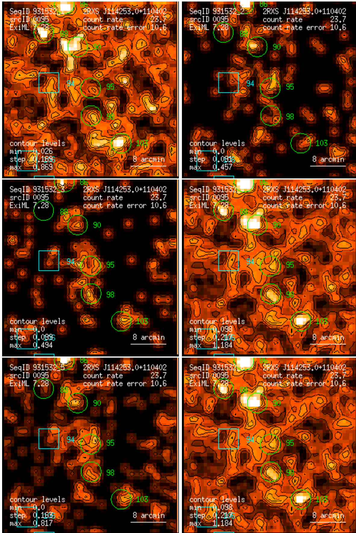
Figure 95: RASS 931532: detection 0095: band rate images, Gaussian filter: (1) PSPC channels 11 – 41, (2) 52 – 90, (3) 91 – 201, (4) 11 – 235, (5) 52 – 201, (6) 11 – 201. Broad band rates in counts/ks. Band rate contour levels in counts/ks/arcmin 2 .
