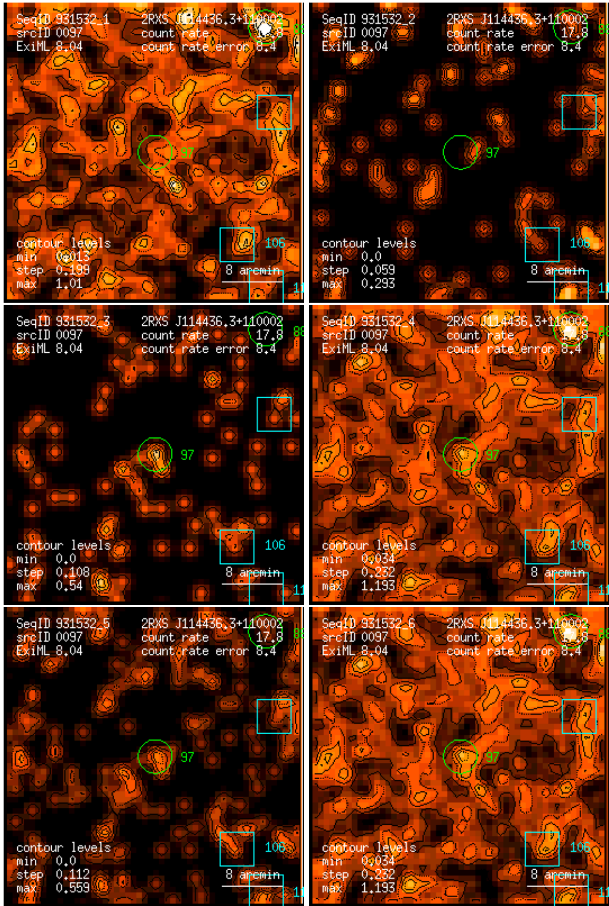
Figure 97: RASS 931532: detection 0097: band rate images, Gaussian filter: (1) PSPC channels 11 – 41, (2) 52 – 90, (3) 91 – 201, (4) 11 – 235, (5) 52 – 201, (6) 11 – 201. Broad band rates in counts/ks. Band rate contour levels in counts/ks/arcmin 2 .
