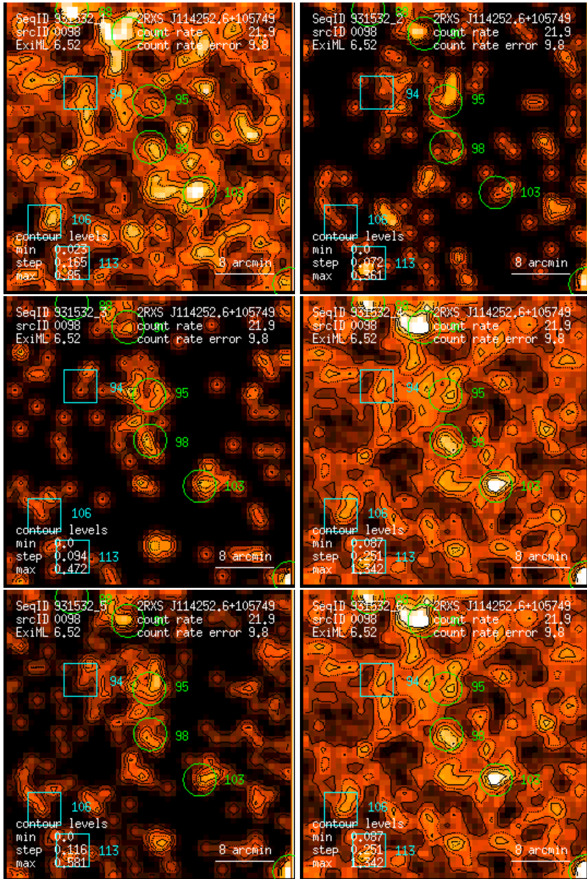
Figure 98: RASS 931532: detection 0098: band rate images, Gaussian filter: (1) PSPC channels 11 – 41, (2) 52 – 90, (3) 91 – 201, (4) 11 – 235, (5) 52 – 201, (6) 11 – 201. Broad band rates in counts/ks. Band rate contour levels in counts/ks/arcmin 2 .
