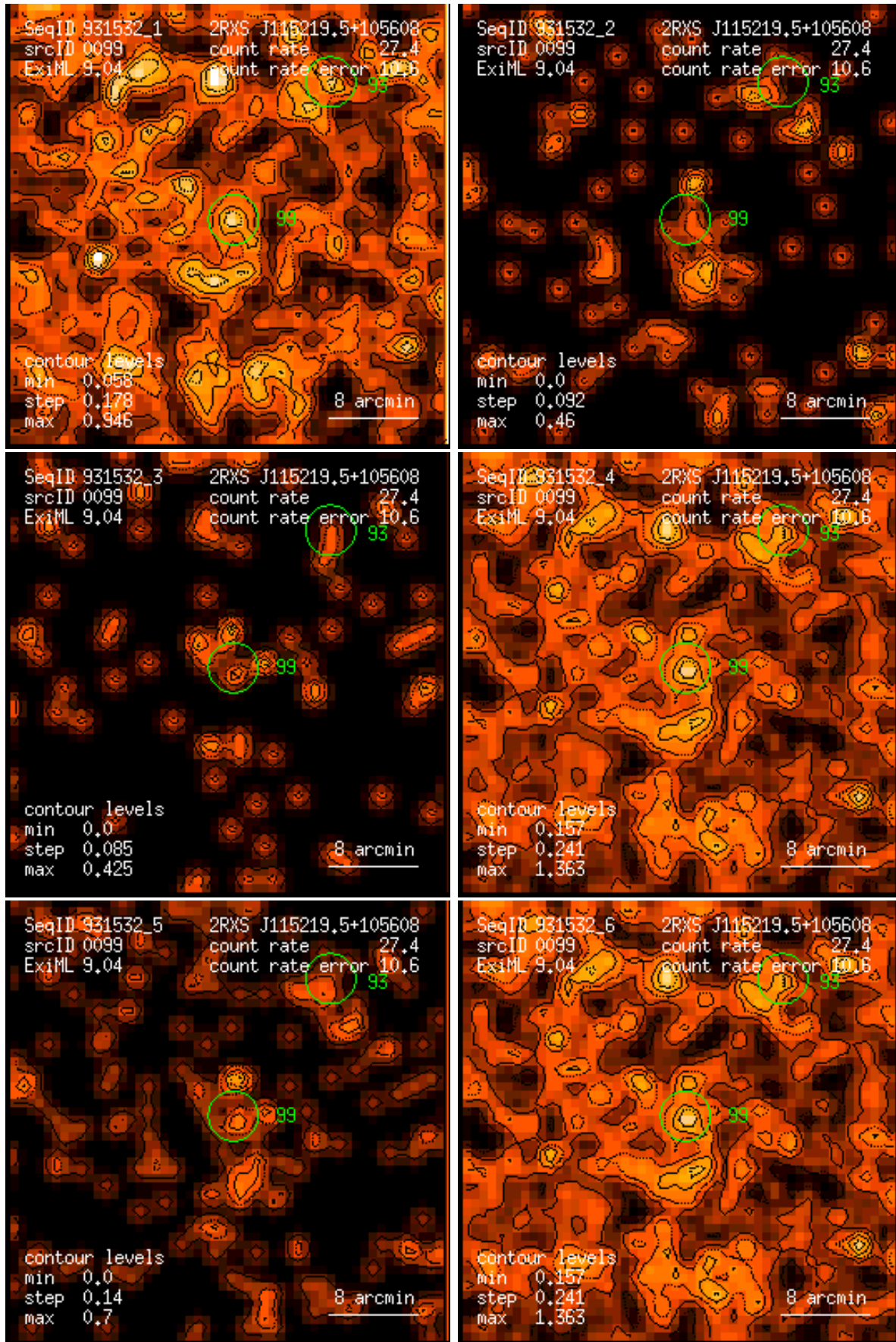
Figure 99: RASS 931532: detection 0099: band rate images, Gaussian filter: (1) PSPC channels 11 – 41, (2) 52 – 90, (3) 91 – 201, (4) 11 – 235, (5) 52 – 201, (6) 11 – 201. Broad band rates in counts/ks. Band rate contour levels in counts/ks/arcmin 2 .
