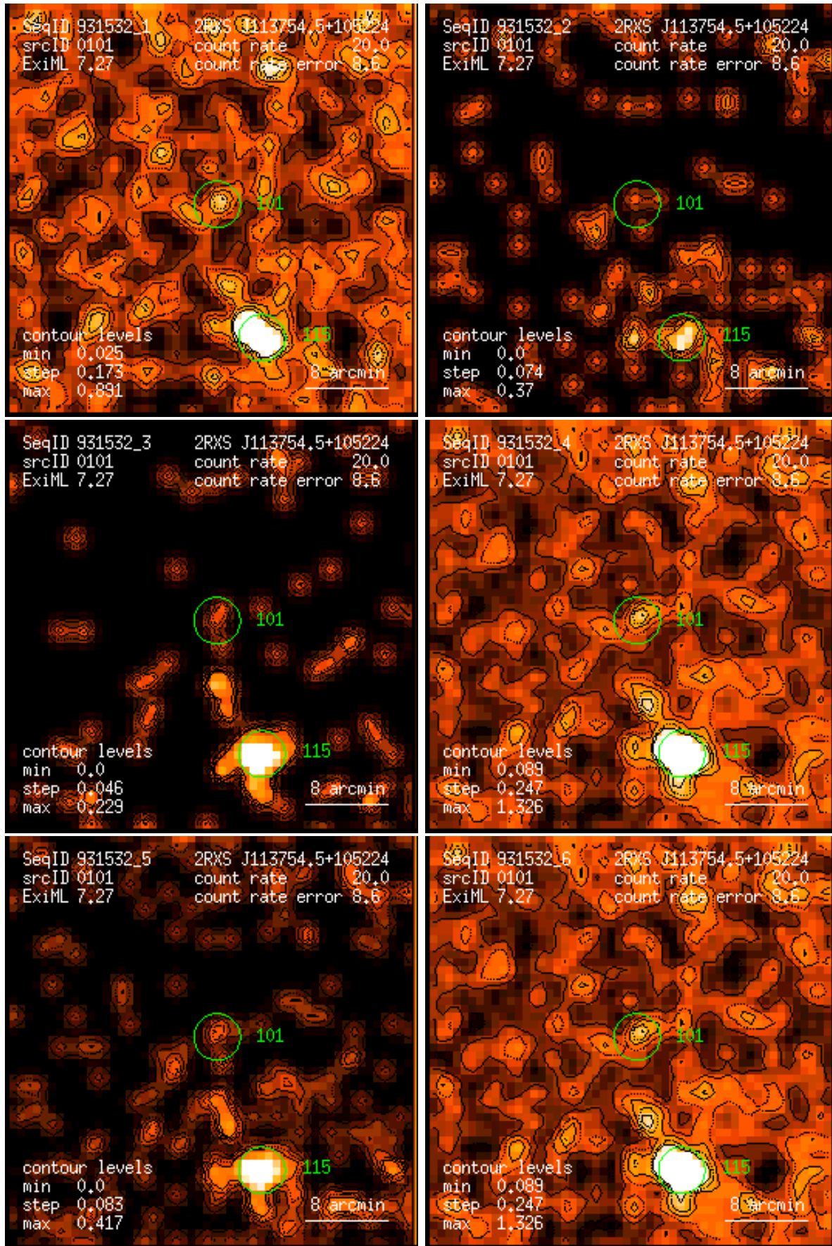
Figure 101: RASS 931532: detection 0101: band rate images, Gaussian filter: (1) PSPC channels 11 – 41, (2) 52 – 90, (3) 91 – 201, (4) 11 – 235, (5) 52 – 201, (6) 11 – 201. Broad band rates in counts/ks. Band rate contour levels in counts/ks/arcmin 2 .
