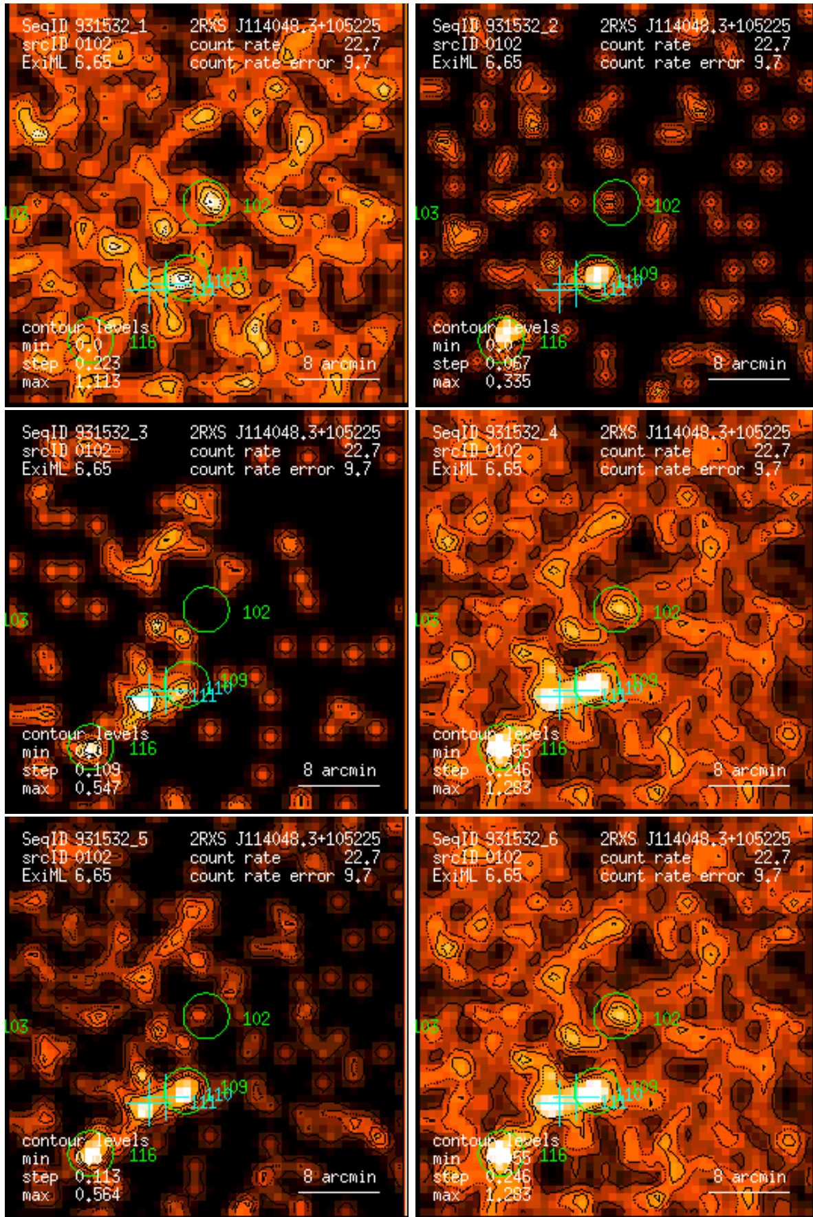
Figure 102: RASS 931532: detection 0102: band rate images, Gaussian filter: (1) PSPC channels 11 – 41, (2) 52 – 90, (3) 91 – 201, (4) 11 – 235, (5) 52 – 201, (6) 11 – 201. Broad band rates in counts/ks. Band rate contour levels in counts/ks/arcmin 2 .
