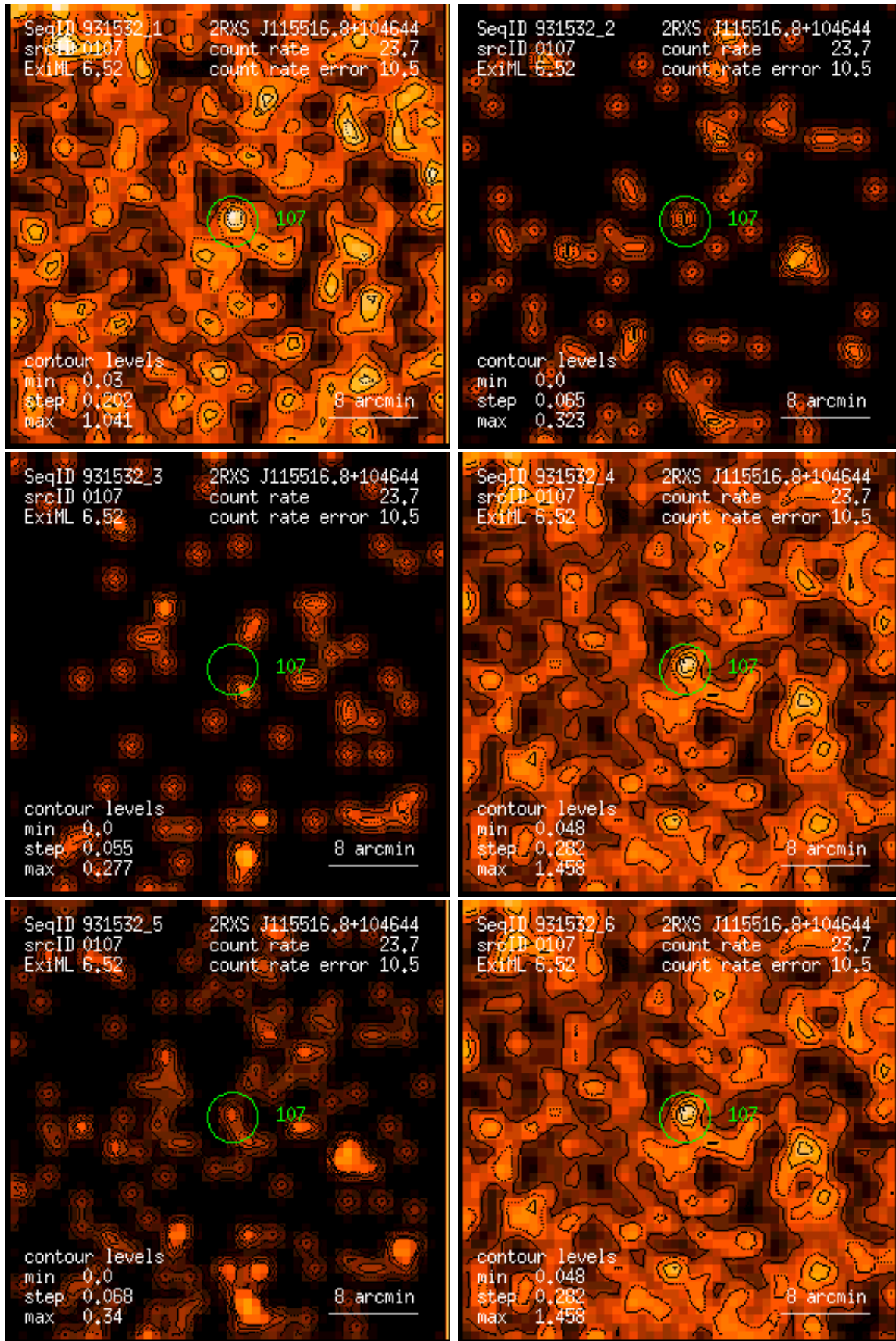
Figure 107: RASS 931532: detection 0107: band rate images, Gaussian filter: (1) PSPC channels 11 – 41, (2) 52 – 90, (3) 91 – 201, (4) 11 – 235, (5) 52 – 201, (6) 11 – 201. Broad band rates in counts/ks. Band rate contour levels in counts/ks/arcmin 2 .
