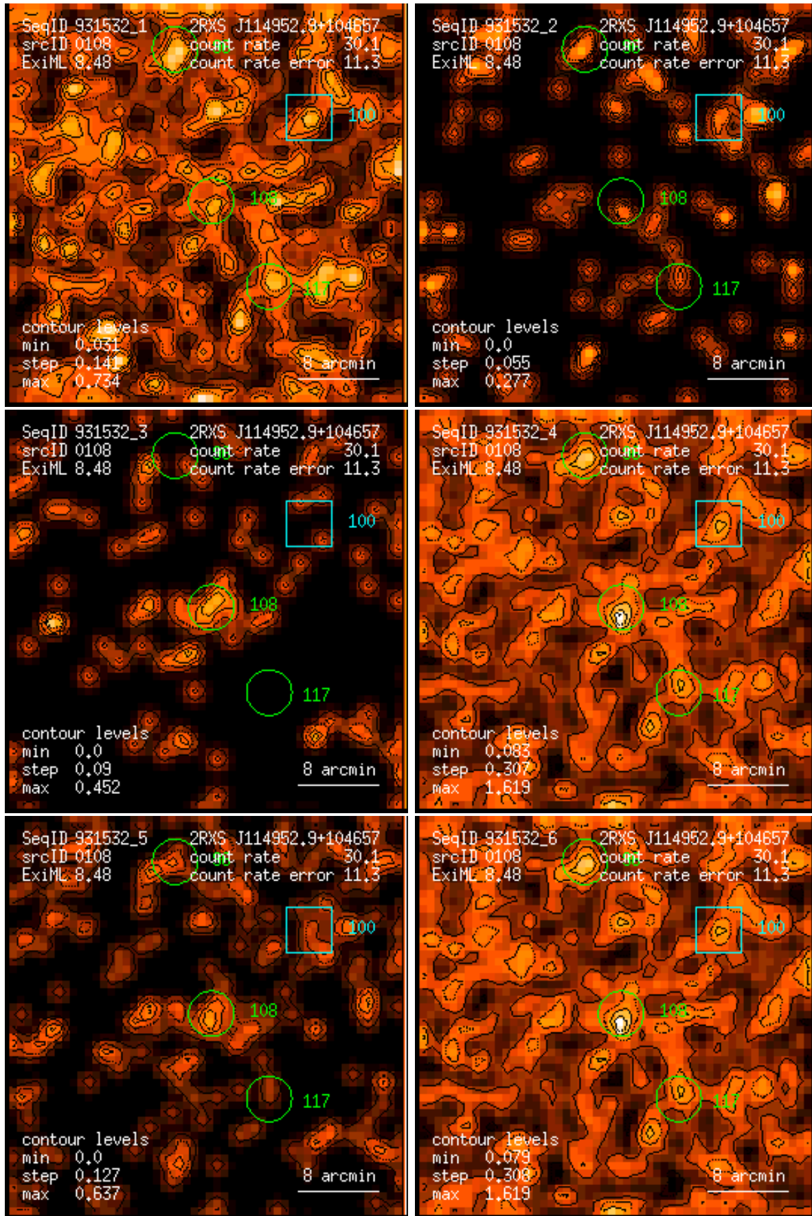
Figure 108: RASS 931532: detection 0108: band rate images, Gaussian filter: (1) PSPC channels 11 – 41, (2) 52 – 90, (3) 91 – 201, (4) 11 – 235, (5) 52 – 201, (6) 11 – 201. Broad band rates in counts/ks. Band rate contour levels in counts/ks/arcmin 2 .
