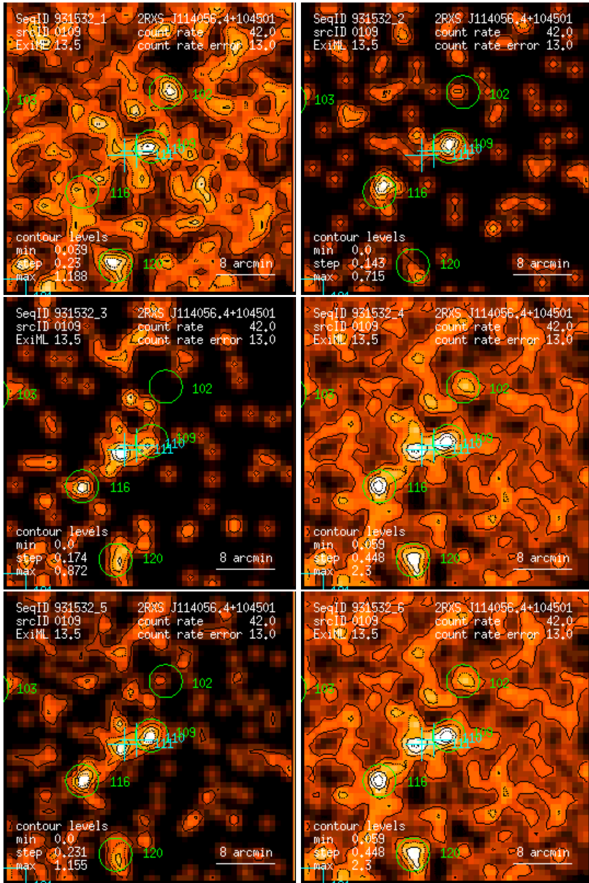
Figure 109: RASS 931532: detection 0109: band rate images, Gaussian filter: (1) PSPC channels 11 – 41, (2) 52 – 90, (3) 91 – 201, (4) 11 – 235, (5) 52 – 201, (6) 11 – 201. Broad band rates in counts/ks. Band rate contour levels in counts/ks/arcmin 2 .
