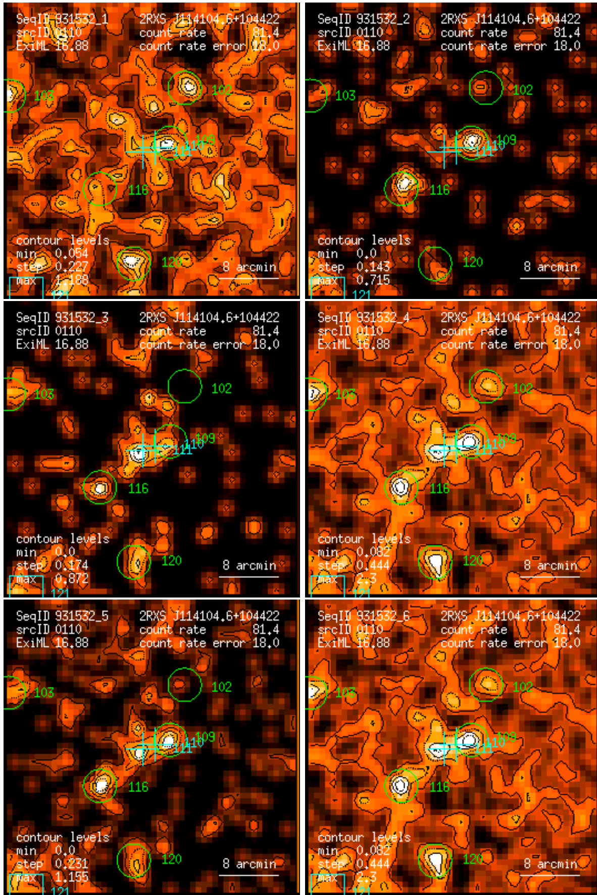
Figure 110: RASS 931532: detection 0110: band rate images, Gaussian filter: (1) PSPC channels 11 – 41, (2) 52 – 90, (3) 91 – 201, (4) 11 – 235, (5) 52 – 201, (6) 11 – 201. Broad band rates in counts/ks. Band rate contour levels in counts/ks/arcmin 2 .
