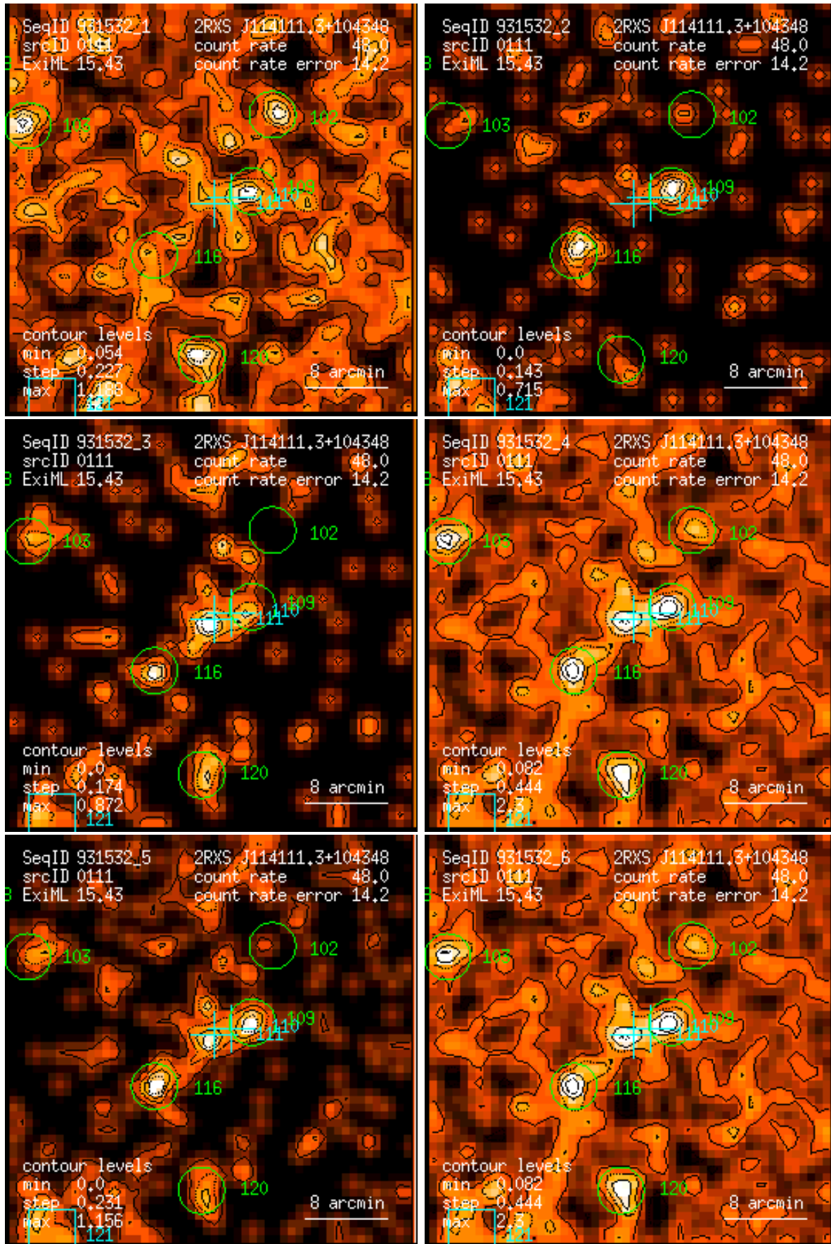
Figure 111: RASS 931532: detection 0111: band rate images, Gaussian filter: (1) PSPC channels 11 – 41, (2) 52 – 90, (3) 91 – 201, (4) 11 – 235, (5) 52 – 201, (6) 11 – 201. Broad band rates in counts/ks. Band rate contour levels in counts/ks/arcmin 2 .
