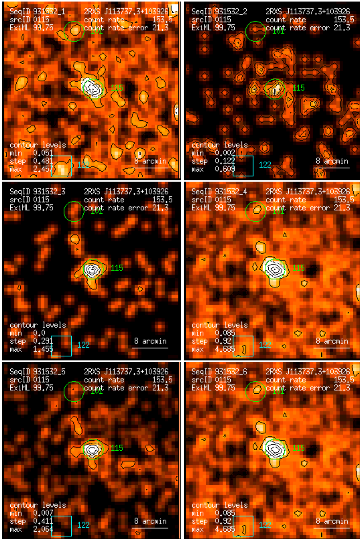
Figure 115: RASS 931532: detection 0115: band rate images, Gaussian filter: (1) PSPPC channels 11 – 41, (2) 52 – 90, (3) 91 – 201, (4) 11 – 235, (5) 52 – 201, (6) 11 – 201. Broad band rates in counts/ks. Band rate contour levels in counts/ks/arcmin 2 .
