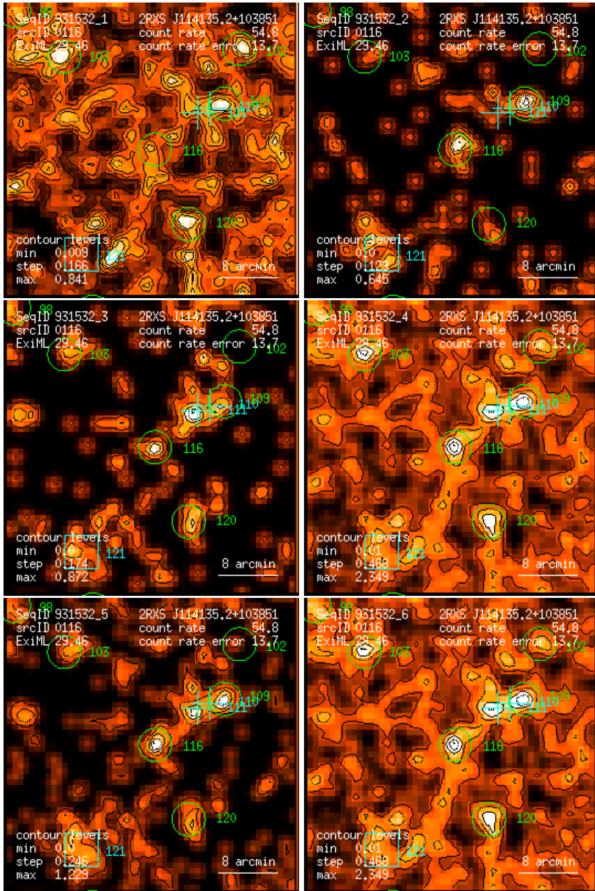
Figure 116: RASS 931532: detection 0116: band rate images, Gaussian filter: (1) PSPC channels 11 – 41, (2) 52 – 90, (3) 91 – 201, (4) 11 – 235, (5) 52 – 201, (6) 11 – 201. Broad band rates in counts/ks. Band rate contour levels in counts/ks/arcmin 2 .
