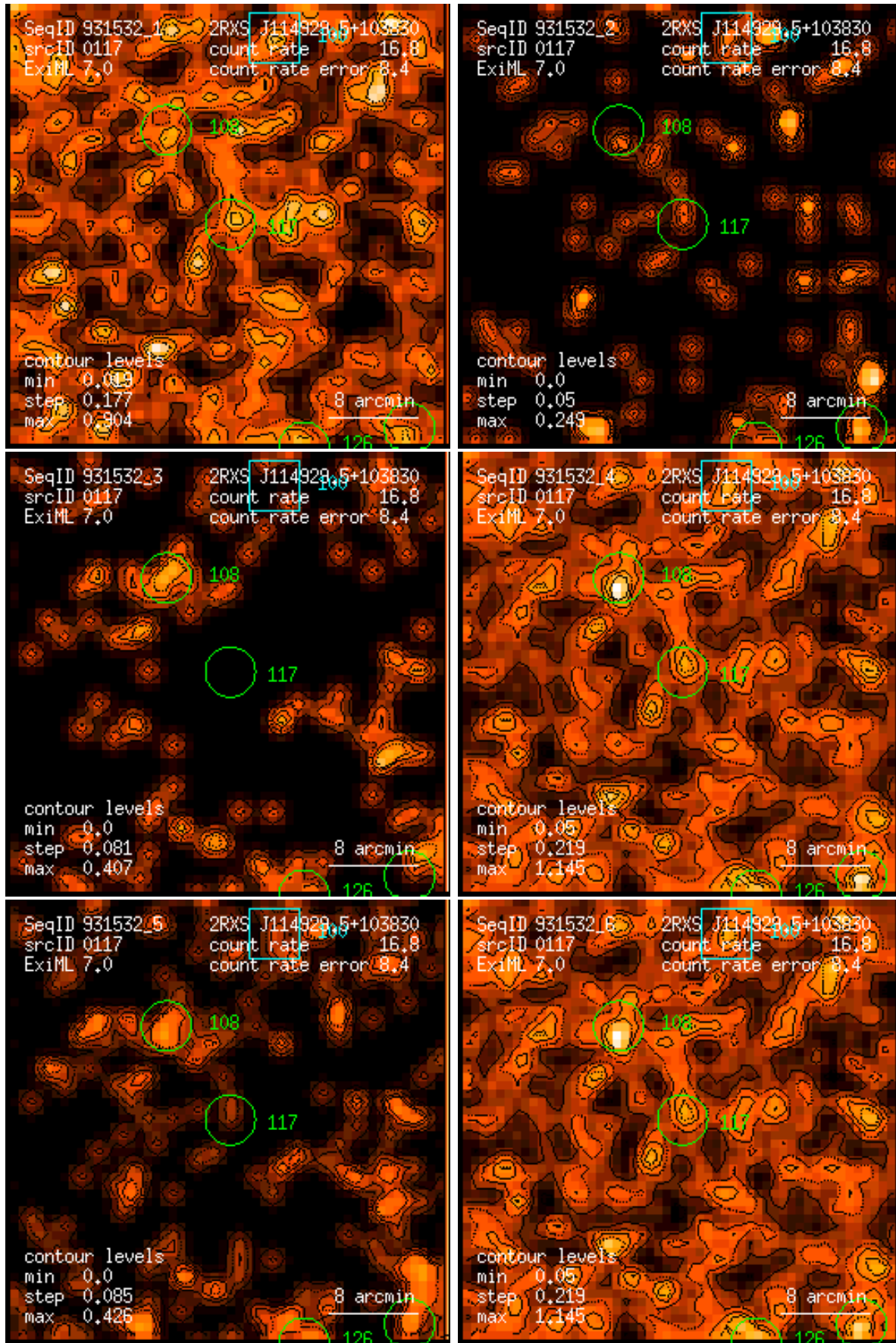
Figure 117: RASS 931532: detection 0117: band rate images, Gaussian filter: (1) PSPC channels 11 – 41, (2) 52 – 90, (3) 91 – 201, (4) 11 – 235, (5) 52 – 201, (6) 11 – 201. Broad band rates in counts/ks. Band rate contour levels in counts/ks/arcmin 2 .
