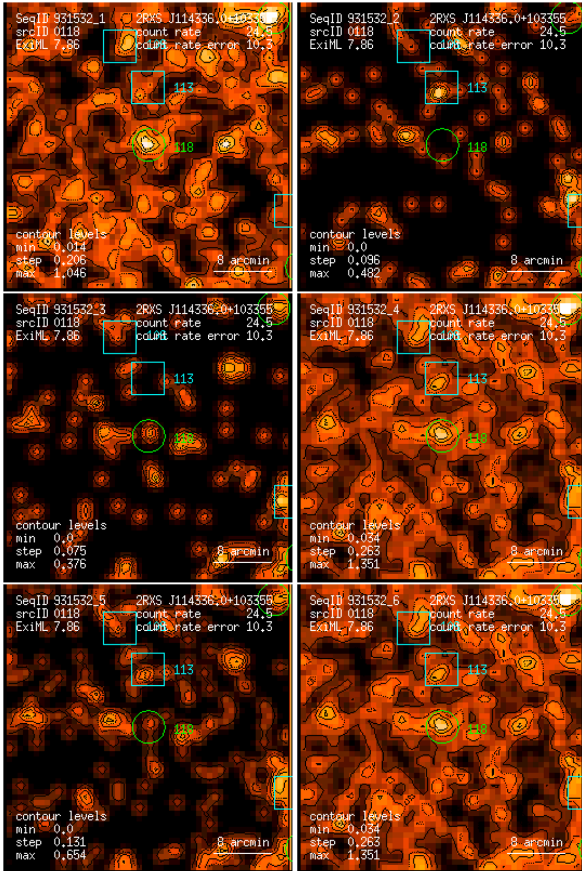
Figure 118: RASS 931532: detection 0118: band rate images, Gaussian filter: (1) PSPC channels 11 – 41, (2) 52 – 90, (3) 91 – 201, (4) 11 – 235, (5) 52 – 201, (6) 11 – 201. Broad band rates in counts/ks. Band rate contour levels in counts/ks/arcmin 2 .
