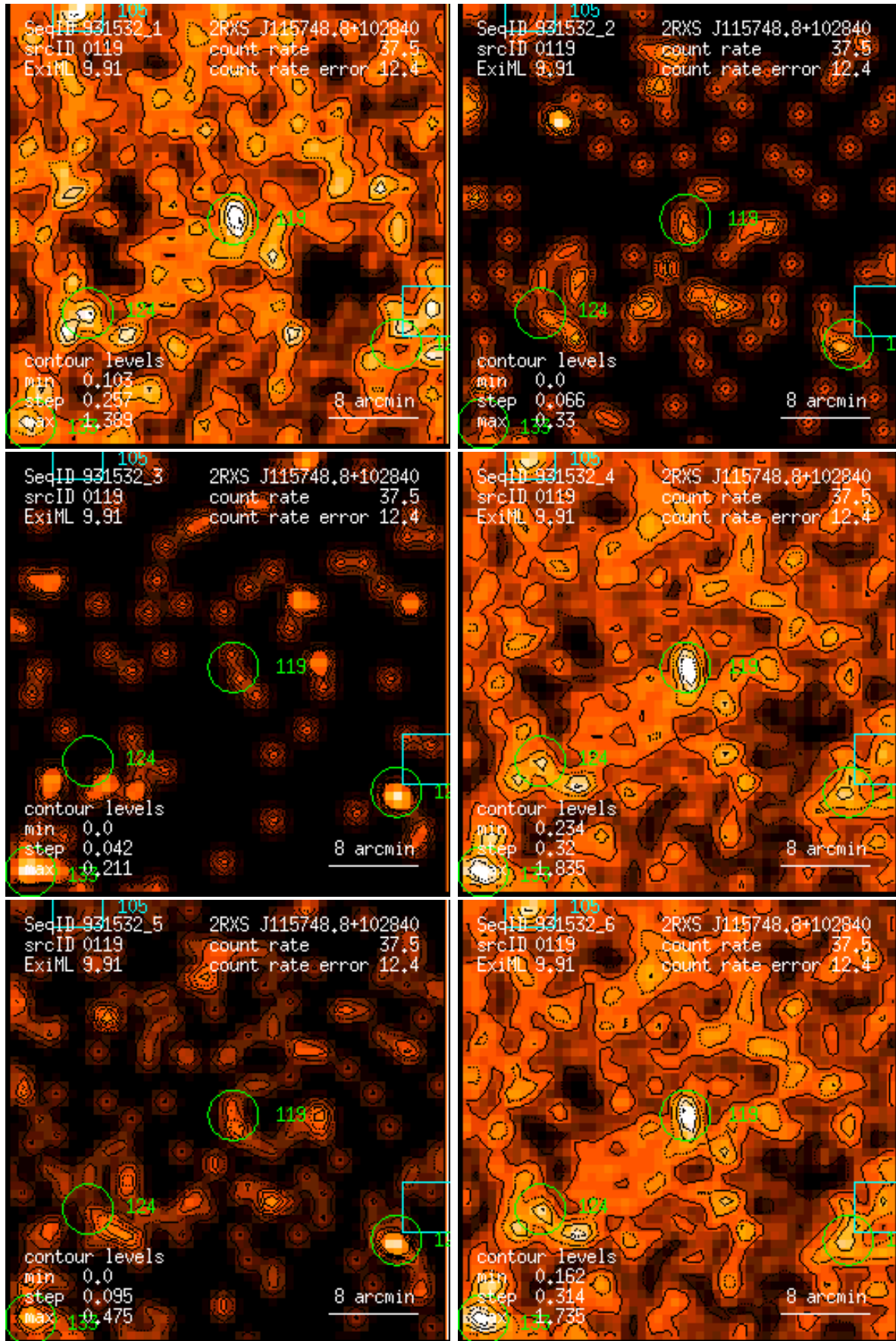
Figure 119: RASS 931532: detection 0119: band rate images, Gaussian filter: (1) PSPC channels 11 – 41, (2) 52 – 90, (3) 91 – 201, (4) 11 – 235, (5) 52 – 201, (6) 11 – 201. Broad band rates in counts/ks. Band rate contour levels in counts/ks/arcmin 2 .
