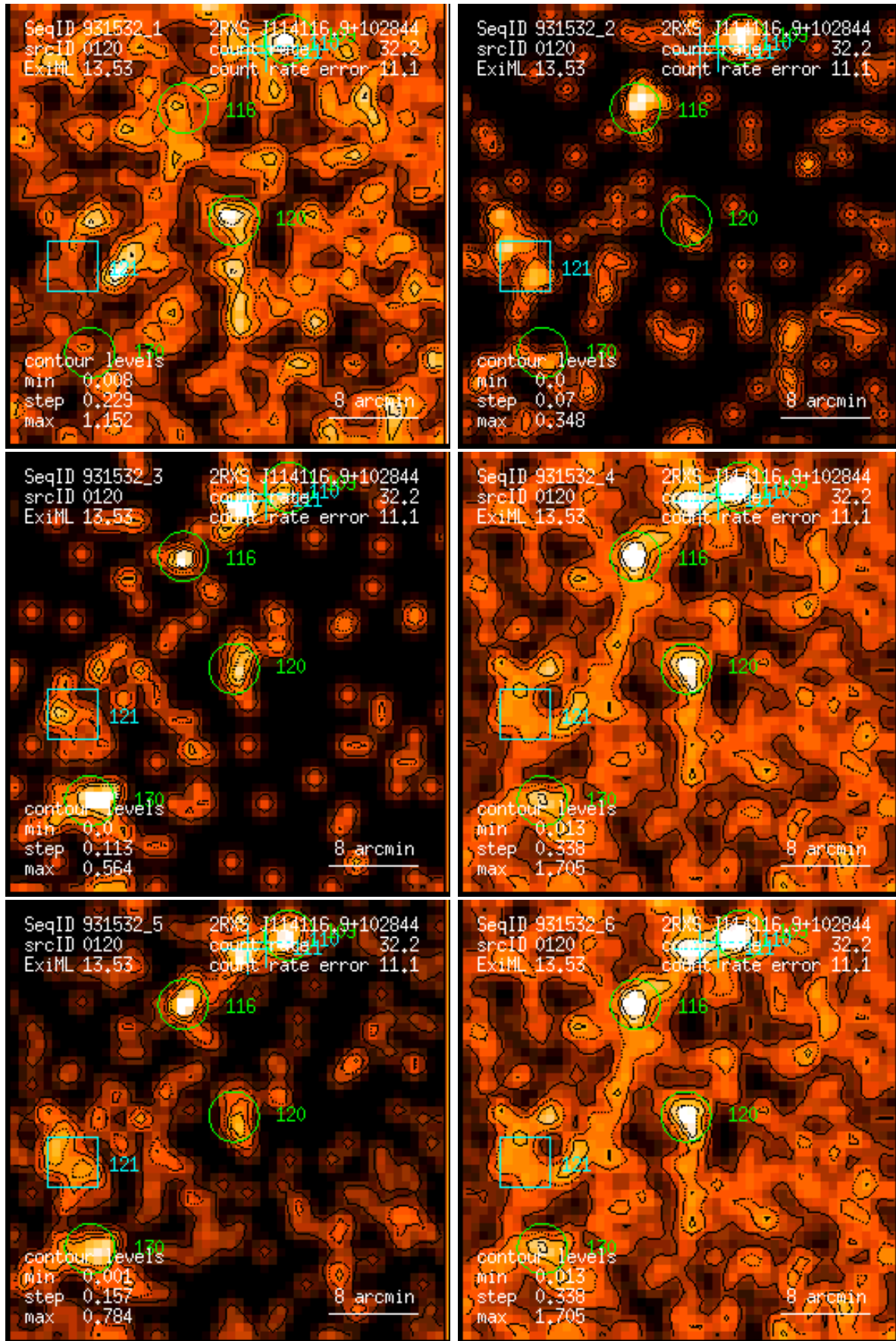
Figure 120: RASS 931532: detection 0120: band rate images, Gaussian filter: (1) PSPC channels 11 – 41, (2) 52 – 90, (3) 91 – 201, (4) 11 – 235, (5) 52 – 201, (6) 11 – 201. Broad band rates in counts/ks. Band rate contour levels in counts/ks/arcmin 2 .
