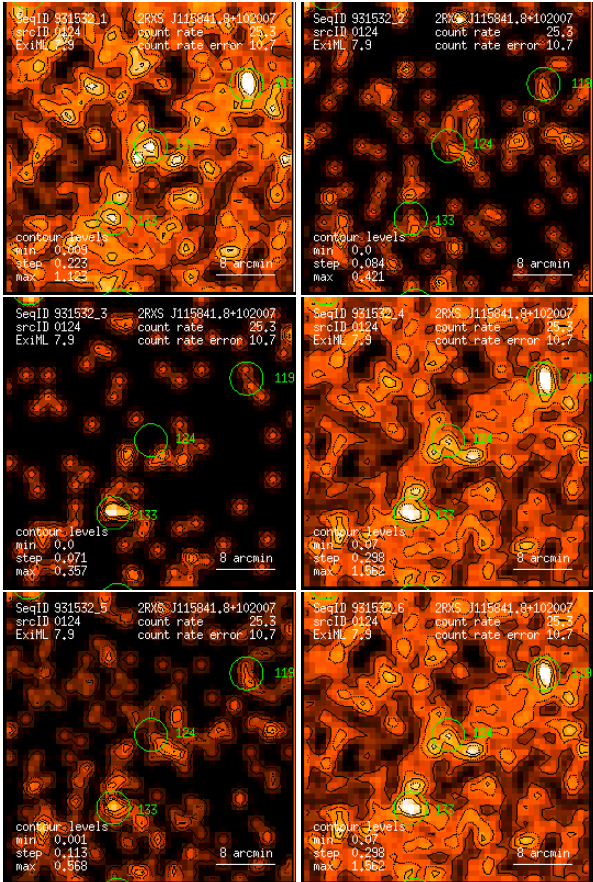
Figure 124: RASS 931532: detection 0124: band rate images, Gaussian filter: (1) PSPC channels 11 – 41, (2) 52 – 90, (3) 91 – 201, (4) 11 – 235, (5) 52 – 201, (6) 11 – 201. Broad band rates in counts/ks. Band rate contour levels in counts/ks/arcmin 2 .
