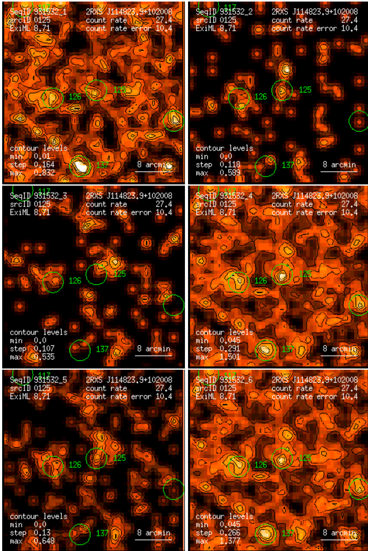
Figure 125: RASS 931532: detection 0125: band rate images, Gaussian filter: (1) PSPC channels 11 – 41, (2) 52 – 90, (3) 91 – 201, (4) 11 – 235, (5) 52 – 201, (6) 11 – 201. Broad band rates in counts/ks. Band rate contour levels in counts/ks/arcmin 2 .
