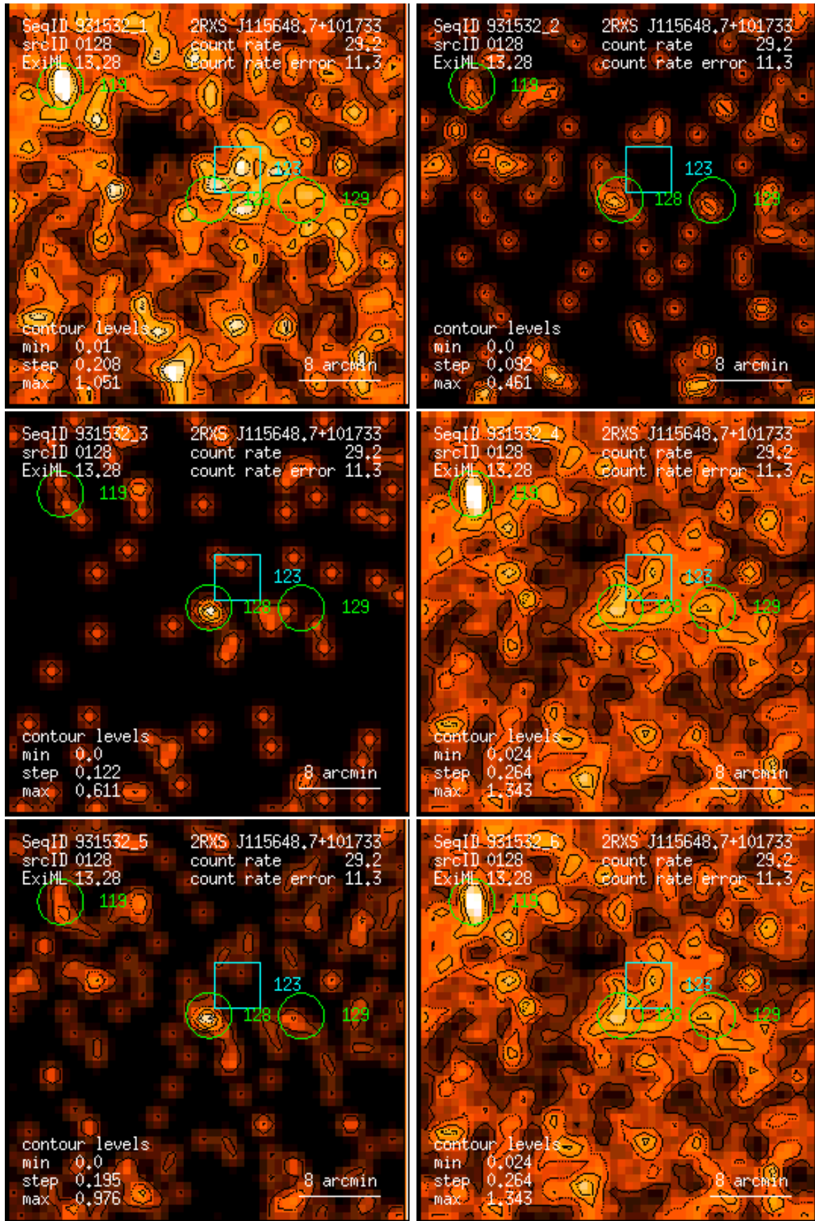
Figure 128: RASS 931532: detection 0128: band rate images, Gaussian filter: (1) PSPC channels 11 – 41, (2) 52 – 90, (3) 91 – 201, (4) 11 – 235, (5) 52 – 201, (6) 11 – 201. Broad band rates in counts/ks. Band rate contour levels in counts/ks/arcmin 2 .
