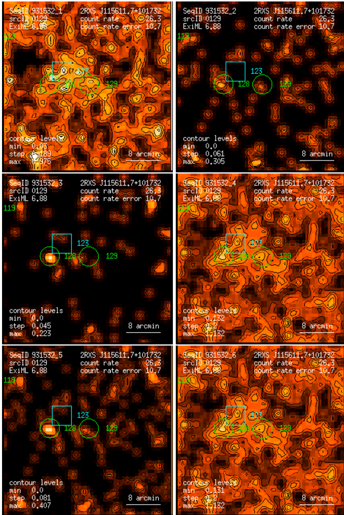
Figure 129: RASS 931532: detection 0129: band rate images, Gaussian filter: (1) PSPC channels 11 – 41, (2) 52 – 90, (3) 91 – 201, (4) 11 – 235, (5) 52 – 201, (6) 11 – 201. Broad band rates in counts/ks. Band rate contour levels in counts/ks/arcmin 2 .
