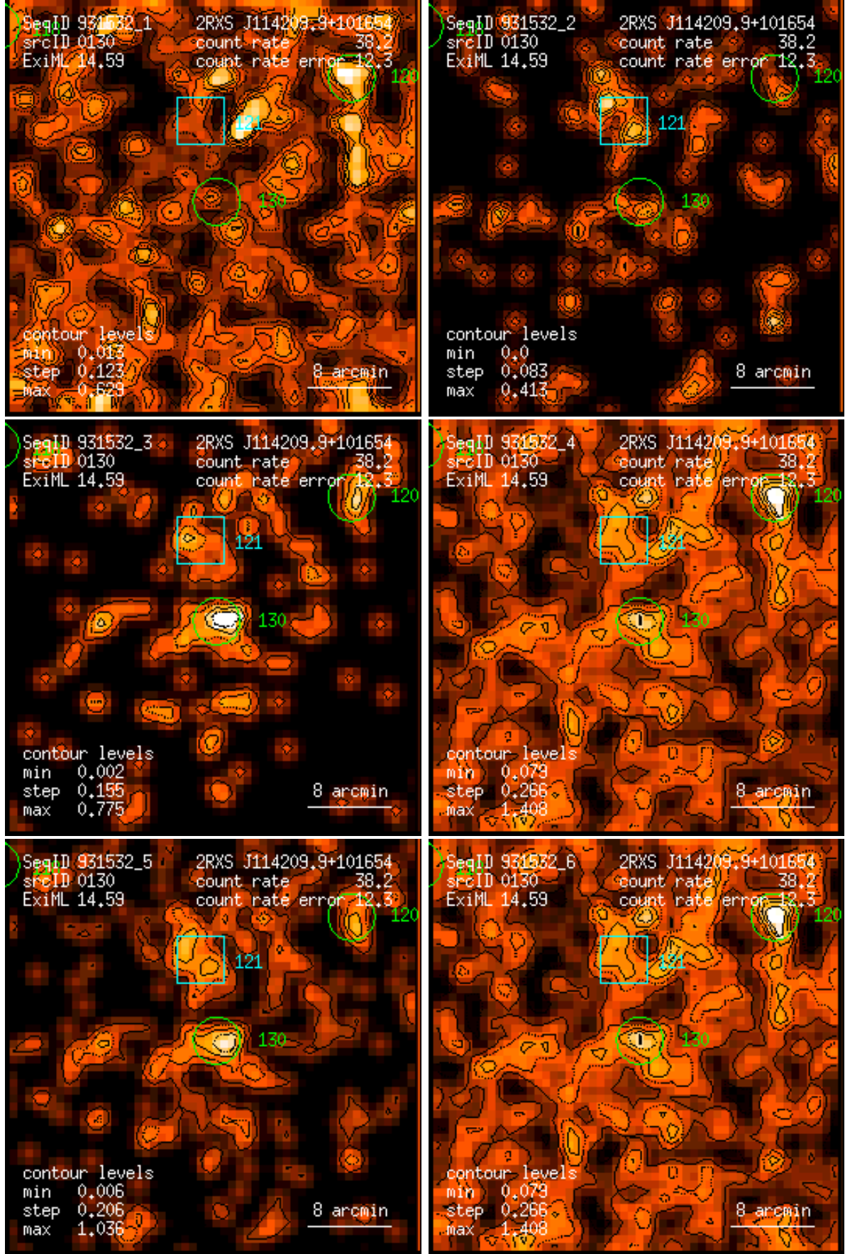
Figure 130: RASS 931532: detection 0130: band rate images, Gaussian filter: (1) PSPC channels 11 – 41, (2) 52 – 90, (3) 91 – 201, (4) 11 – 235, (5) 52 – 201, (6) 11 – 201. Broad band rates in counts/ks. Band rate contour levels in counts/ks/arcmin 2 .
