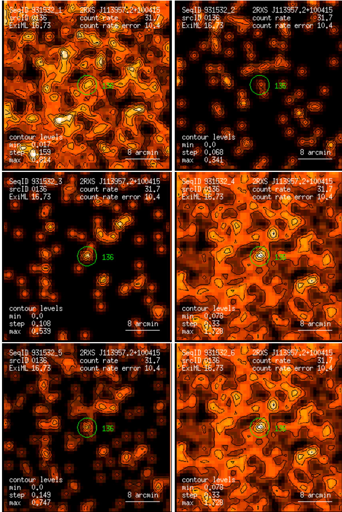
Figure 136: RASS 931532: detection 0136: band rate images, Gaussian filter: (1) PSPC channels 11 – 41, (2) 52 – 90, (3) 91 – 201, (4) 11 – 235, (5) 52 – 201, (6) 11 – 201. Broad band rates in counts/ks. Band rate contour levels in counts/ks/arcmin 2 .
